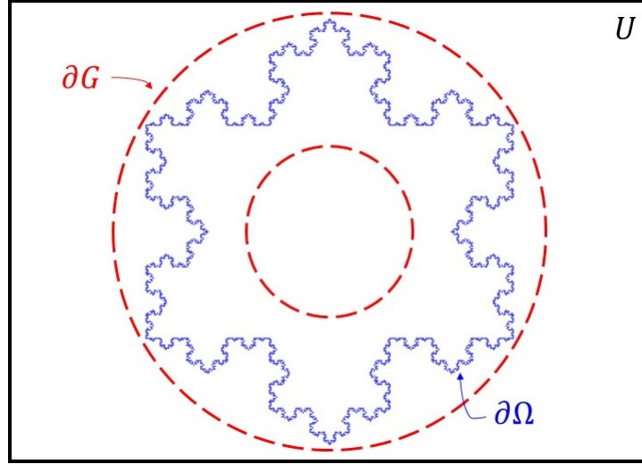
Figure 7: An example of a admissible uniform domain which is not an admissible Lipschitz domain. The domain lies inside the blue Von Koch curve (represented by a fifth generation pre-fractal [source: Wikipedia]) and its boundary is endowed with the \frac{\ln 4}{\ln 3} -dimensional Hausdorff measure. U is the interior of the black rectangle. G lies between the red dashed lines \partial G .
