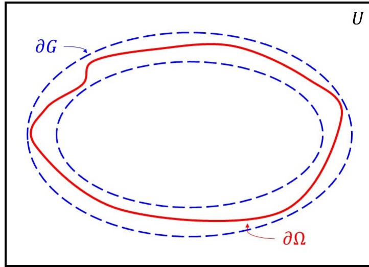
Figure 5: An example of an admissible Lipschitz domain, lying inside the red boundary \partial\Omega . U is the interior of the black rectangle. G lies between the blue dashed lines \partial G .
