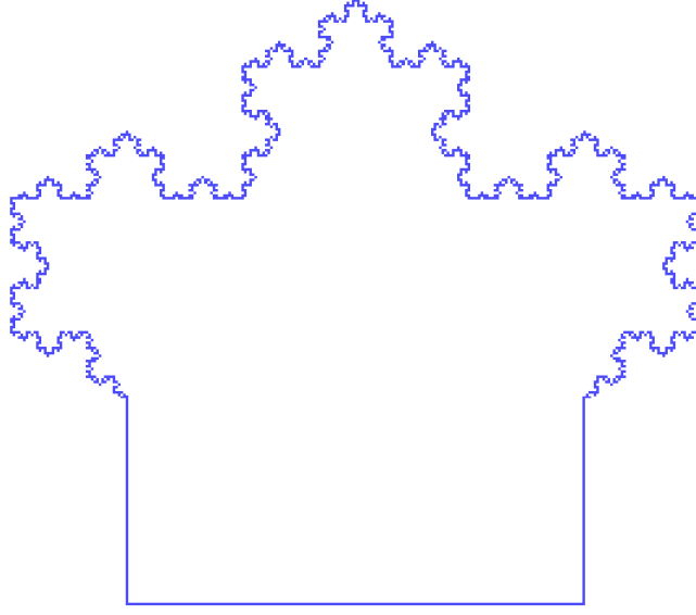
Figure 3: An example of a two-sided admissible domain of \mathbb{R}^2 , lying inside the blue line. The upper part of the boundary is a Von Koch curve, which is a \frac{\ln 4}{\ln 3} -set (represented by a fifth generation pre-fractal [source: Wikipedia]). The lower part consists of a portion of a square, which is Lipschitz. The boundary is endowed with the 1-dimensional Lebesgue measure on the lower part and the \frac{\ln 4}{\ln 3} -dimensional Hausdorff measure on the upper part: condition (2.1) is satisfied for d = 1 .
