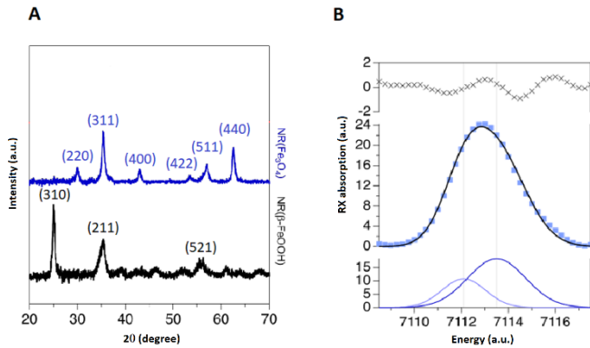
Fig. 3 A) XRD diffractograms of akaganeite (NR( \beta -FeOOH), black line) and magnetite (NR( \text{Fe}_3\text{O}_4 ), blue line) NRs. B) XANES analysis of magnetite NRs (squares: experimental points; black curve: double normal law fit; black crosses: residues; light blue curve: contribution of Fe(II), dark blue curve : contribution of Fe(III)).
