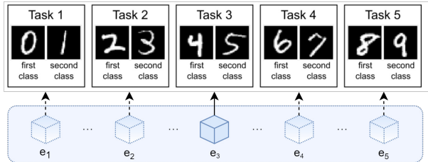
Figure 2: Example of a generated stream in Avalanche, composed by five experiences, implementing the common SplitMNIST benchmark [56]. When accessing experience e_3 , the A_{CL} algorithm has no access to previous or future experiences.
