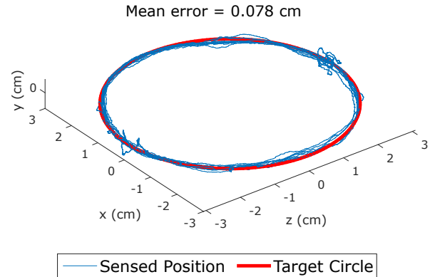
Circle Constraint
