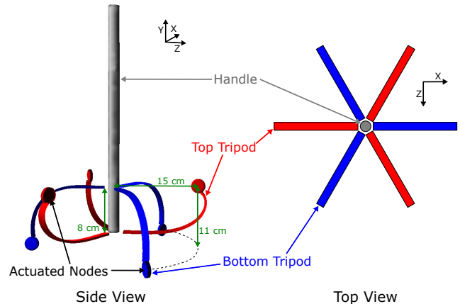
Fig. 2. The device consists of two flexible beam tripod structures attached to the handle and the rigid frame. This schematic shows the bottom (blue) and top (red) tripods as well as the coordinate frame that will be used in the rest of the paper. The parameters shown in the side view, consisting of the distance between handle attachment points, radius to actuated node, and vertical distance between the actuated nodes, are easily adjustable using the device frame and could be used for design optimization. The top view shows how the beams are distributed around the handle.
