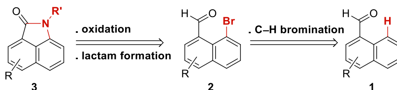
Scheme 1. Retrosynthesis of naphtholactam skeleton thanks to a C–H activation step.
