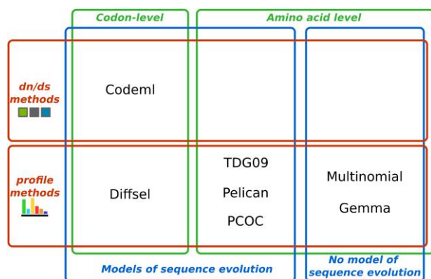
FIG. 2. Methods evaluated in the manuscript. Methods have been positioned based on whether they are based on d_N/d_S or amino-acid profiles, whether they work at the codon or amino-acid level, and whether they rely on a model of sequence evolution running along a phylogeny or not.
