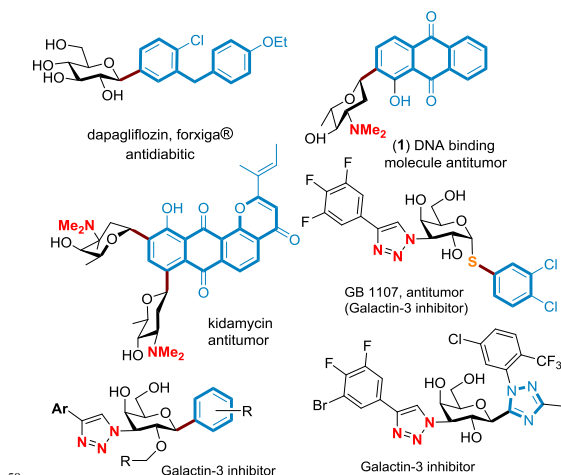
Figure 1. Aryl C-glycosides-based bioactive molecules
