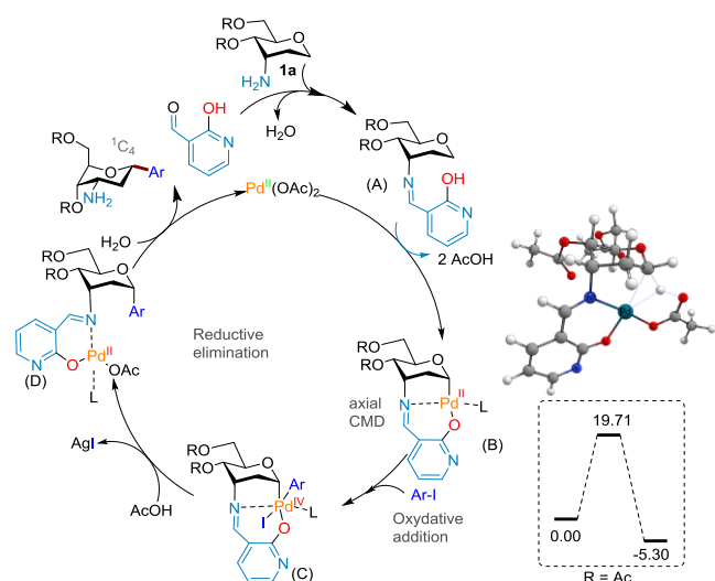
Figure 2. Proposed mechanism and DFT calculations
