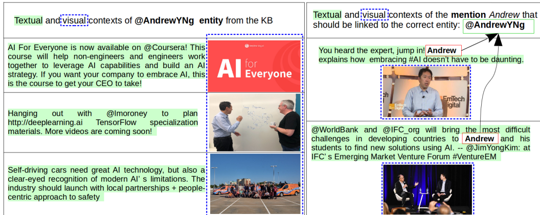
Figure 1: An illustrative example of multimodal Entity Linking on our Twitter dataset. The example depicts a subset of (text, image) pairs representing the entity @AndrewYNg (left), and some example of (text, image) pairs related to the mention Andrew (right).
