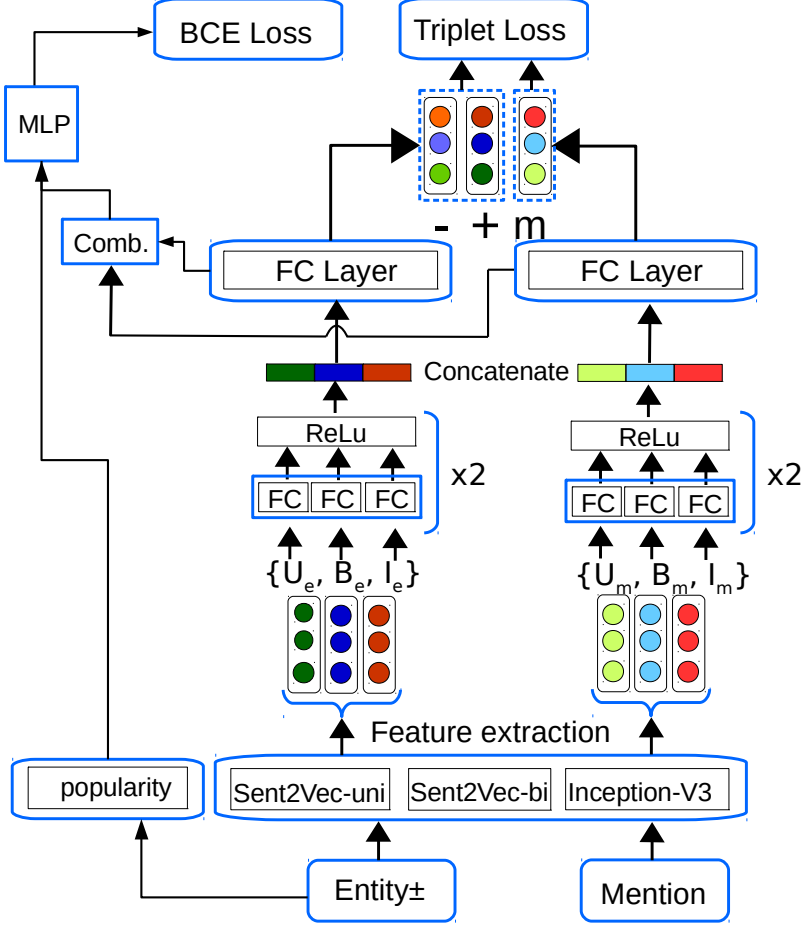
Figure 2: Triplet ranking model for learning entity and mention joint representations.
