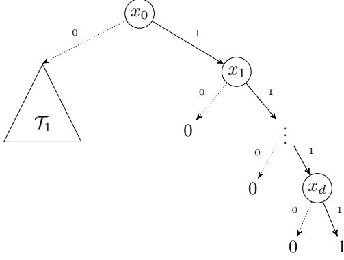
Figure 3: The decision tree \mathcal{T}_2 in the proof of Proposition 2.
