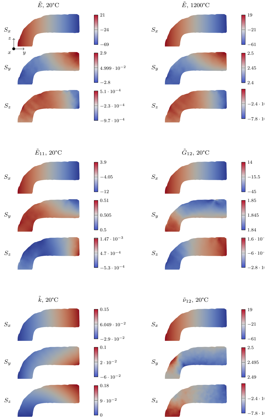
Figure C1: Some sensitivity fields cut in the median plane of the sample: displacement (μm) induced by a variation of the normalised parameters of 1%.
