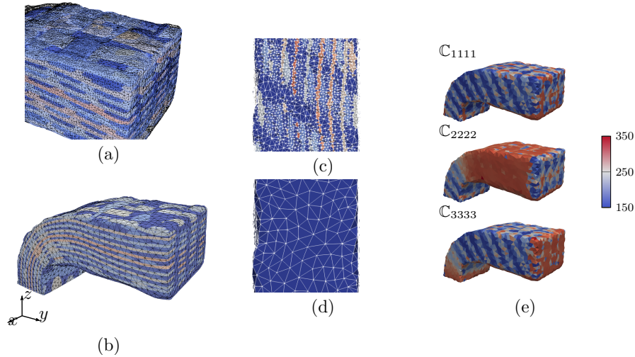
Figure A2: Local meso-to-macro homogenisation. (a) Zoom on the mesoscale mesh, superimposed with the image of the weaving pattern; (b) Macroscale mesh superimposed with the image of the mesostructure. The mesoscale mesh (c), with a mesh size of 90\ \mu\text{m} , is conformal, whereas the macroscale mesh (d), with a mesh size of 225\ \mu\text{m} , is not. (e) Fields of the three first diagonal components of the macroscopic effective stiffness tensor \mathbb{C}_{\text{eff}} (GPa) issued from the local homogenisation.
