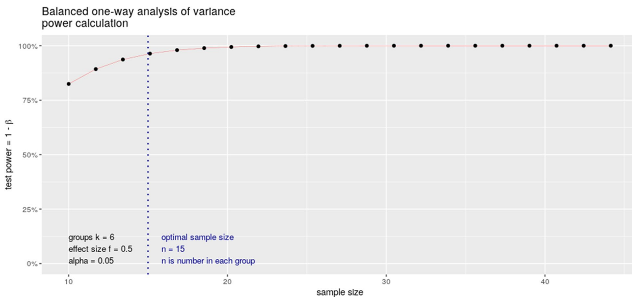
Fig. 2 Power calculation
