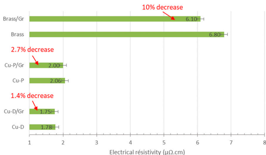
Figure 7. Electrical resistivity measurement at 20°C for various single and composite copper matrix materials.
