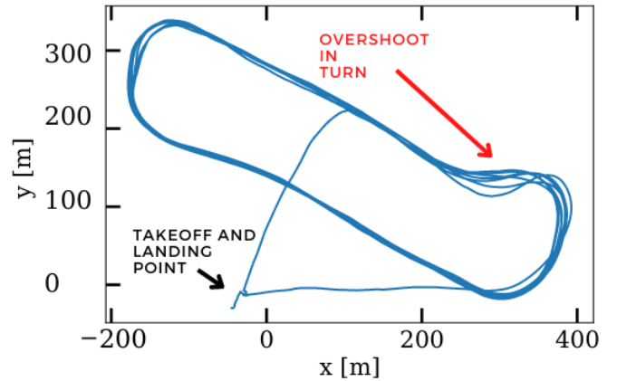
Figure 6: Flight trajectory in the IMAV2022 competition: overshoot in one of the turns caused by strong winds.
