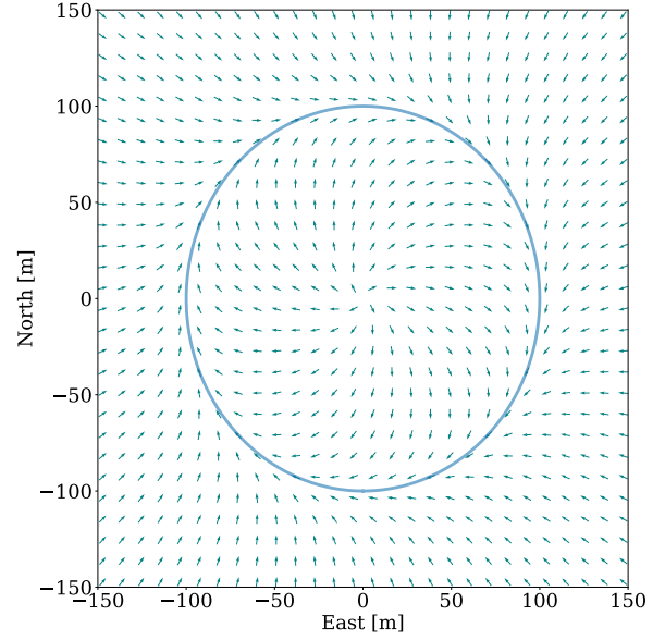
Figure 2: Illustration of vector field guidance, the arrows indicate the velocity direction at each point in the plane.
