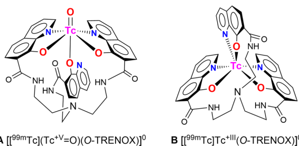
Fig. 6 Proposed structures for the complex [[^{99m}\text{Tc}]\text{Tc-O-TRENOX} : A in the Tc+V oxidation state \{[^{99}\text{Tc}](\text{Tc}=\text{O})^{3+}\} core and B in the Tc+III oxidation state
