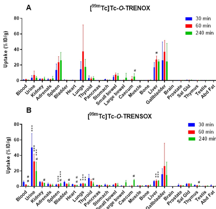
Fig. 4 Biodistribution of [^{99m}\text{Tc}]\text{Tc-O-TRENOX} (A) and [^{99m}\text{Tc}]\text{Tc-O-TREN-SOX} (B) in Swiss mice at 30, 60 and 240 min post-injection. Data are expressed in \% \text{ID/g} as mean \pm SD ( n = 4 / time point). Abd: abdominal; Sal Gld: salivary glands. *: p < 0.05 ; **: p < 0.01 and ***: p < 0.001 versus [^{99m}\text{Tc}]\text{Tc-O-TRENOX} . #: p < 0.05 and ##: p < 0.01 versus 30 min
