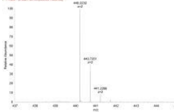
04/03/14/718 RT: 27.27 AV: 1 NL: 3.0804 F: FTMS - c H218 w P-04 m/z (300.00-1600.00)
