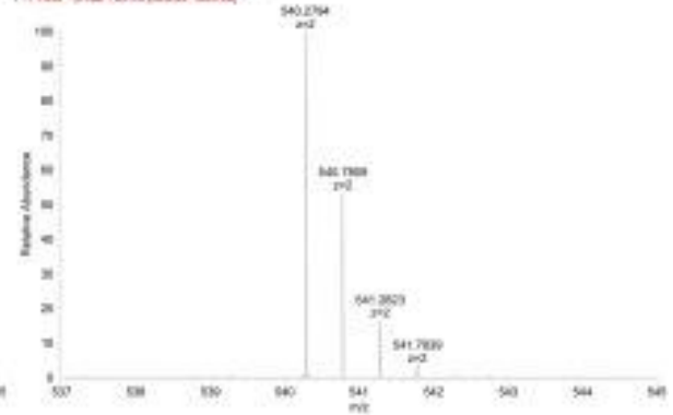
04/03/14/519 RT: 32.80 AV: 1 NL: 5.3884 F: FTMS - c H218 w P-04 m/z (300.00-1600.00)
