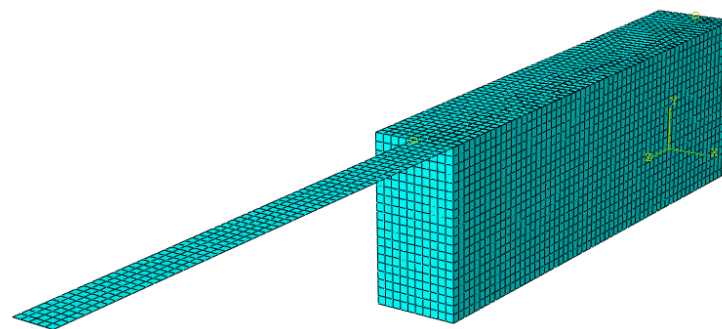
Figure 9. 3D FEM model of single-lap shear test.
