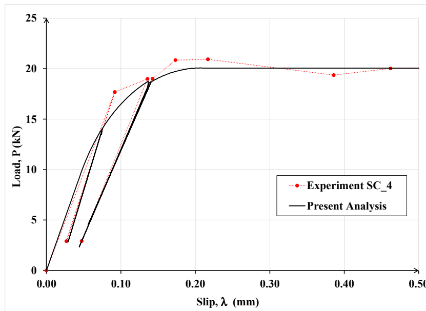
Figure 17. Comparison of experimental and analytical load-slip curves for specimen SC_4 subjected to cyclic load.
