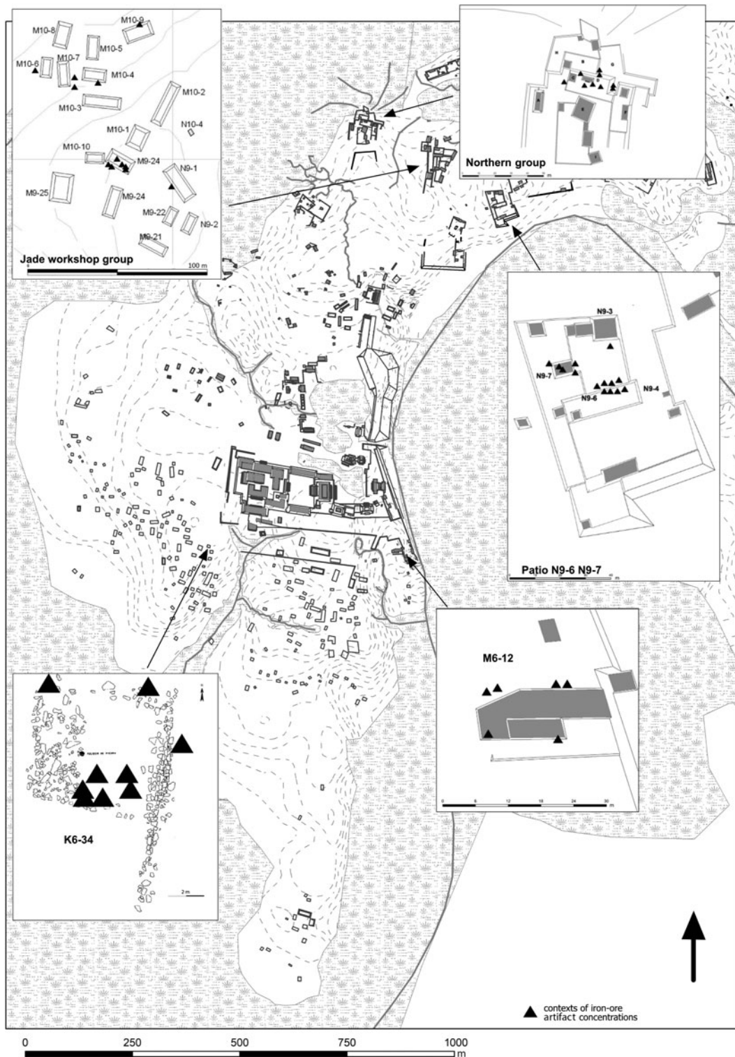
Figure 5. Distribution of the iron-ore artefact concentrations in Cancun. Map by M. Wolf; layout by S. Eliès.
