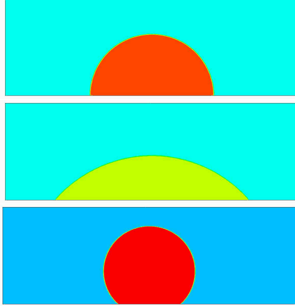
Figure 3. Simulation of the evolution of a drop on a flat surface as a function of the curvature applied to the wall. On top a drop in equilibrium where the curvature \kappa_{\ell} = 1600 and the contact angle \theta_c = 90^\circ are given as initial condition, in the center the curvature \kappa_{\ell} = 750 ( \theta_c = 48.2^\circ ) is imposed on the triple line and at a time of t = 0.2 s we impose \kappa_{\ell} = 2230 ( \theta_c = 150^\circ ).
