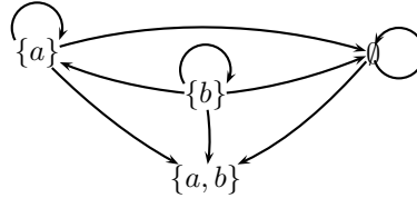
Figure 1. \succeq_2 \subseteq \mathcal{P}(\mathcal{A}) \times \mathcal{P}(\mathcal{A})
