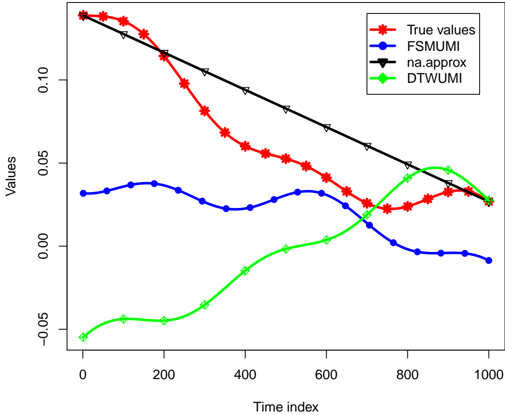
FIGURE 4 Visual comparison of completion data of different imputation approaches with real data on the 1 st signal of synthetic series with the gap size of 1000
