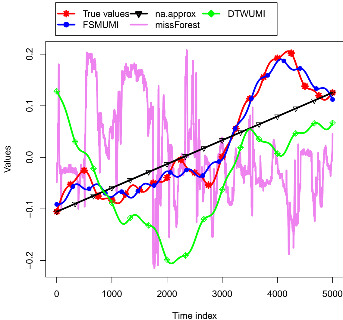
FIGURE 5 Visual comparison of completion data of different imputation approaches with real data on the 1 st signal of synthetic series with the gap size of 5000
