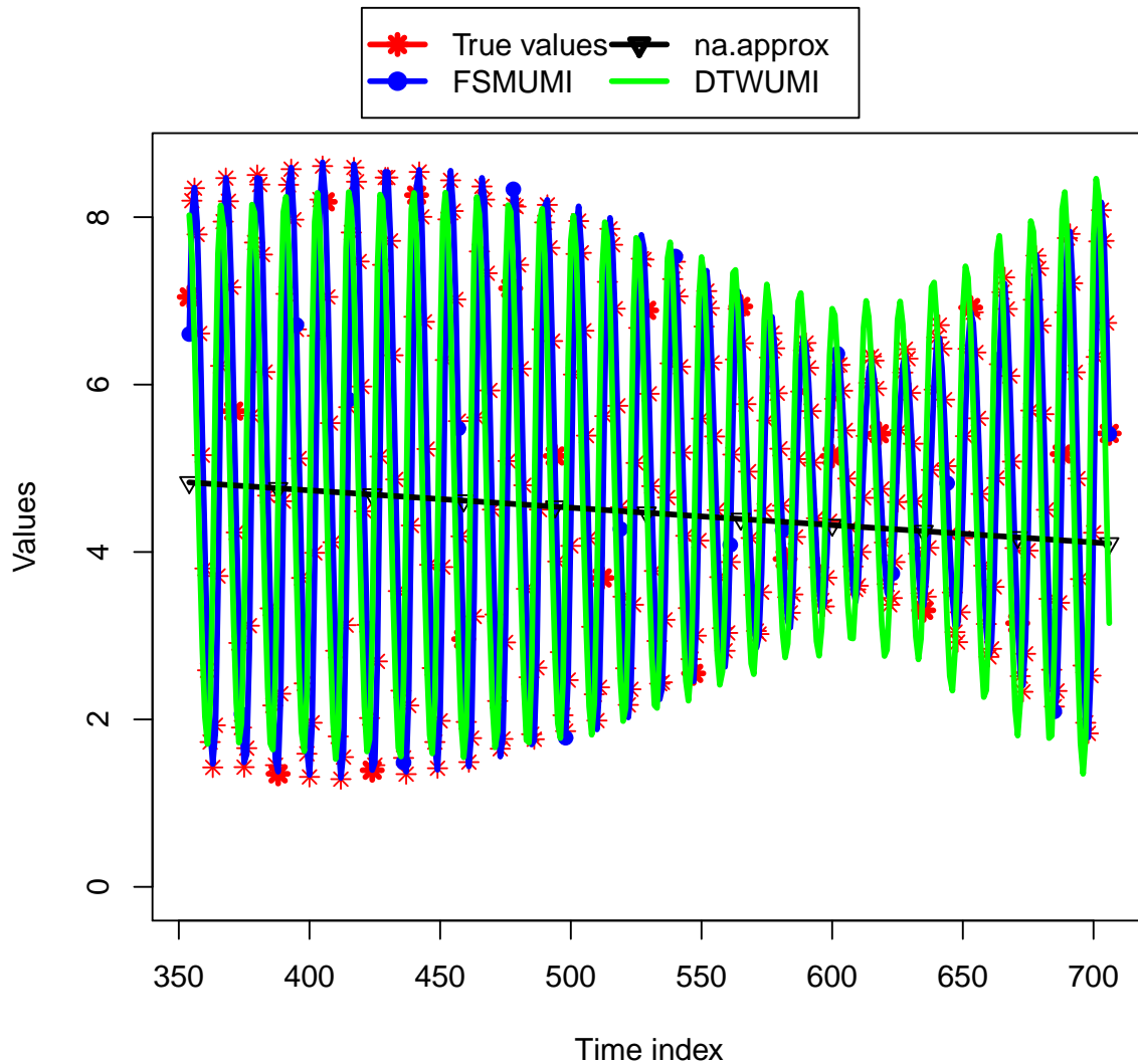
FIGURE 6 Visual comparison of completion data of different imputation approaches with real data on the 2 nd signal of MAREL Carnot dataset with the gap size of 353
