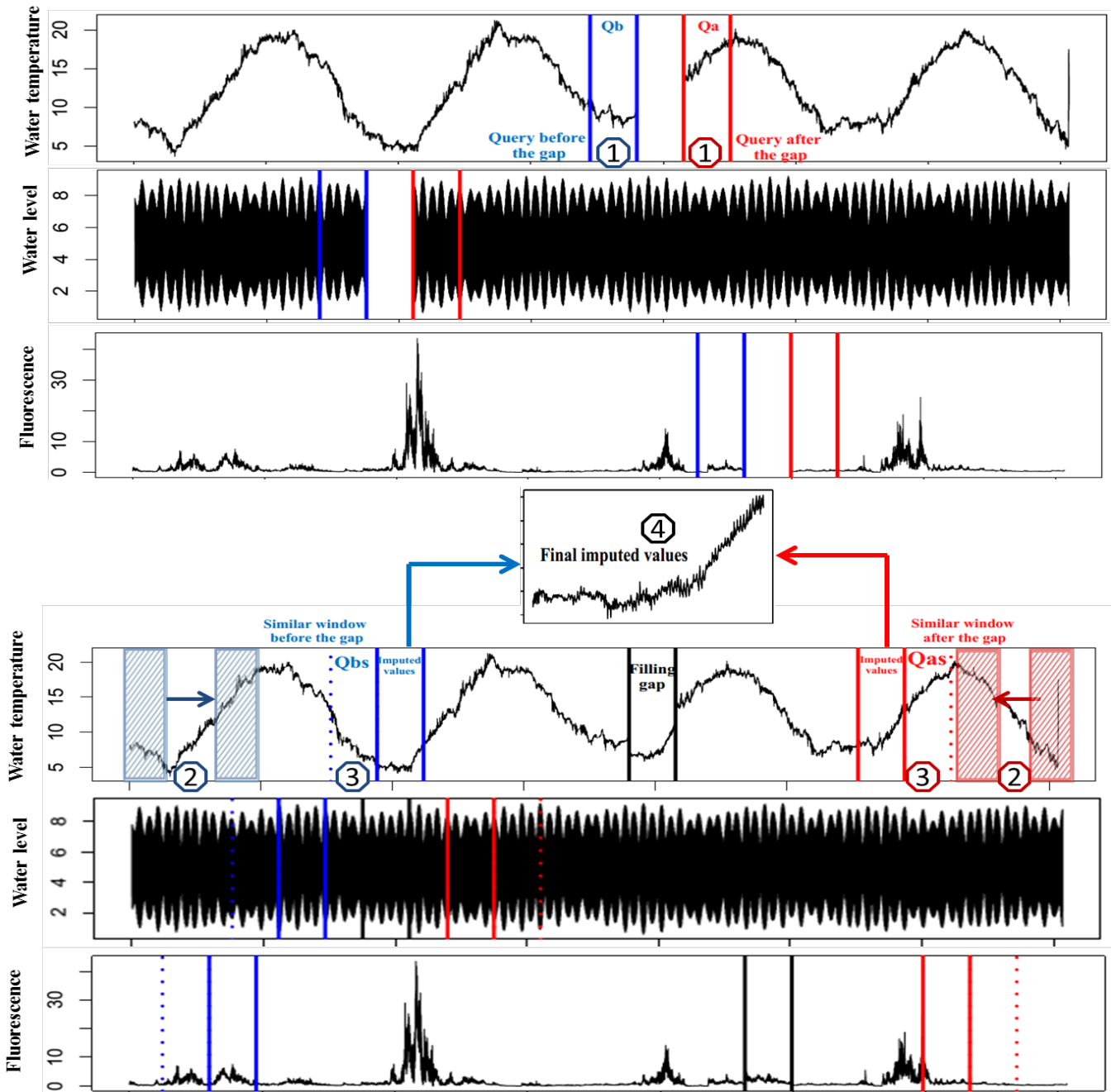
FIGURE 3 Scheme of the completion process: 1- Building queries, 2-Comparing sliding windows, 3-Selecting the most similar windows, 4- Completing gap.
