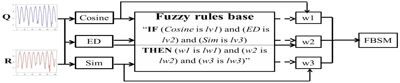
FIGURE 1 Computing scheme of the new similarity measure
