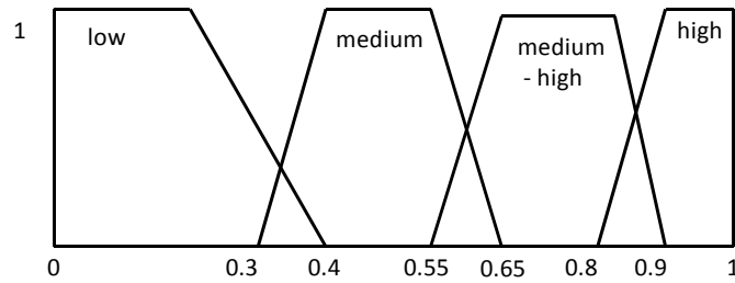
FIGURE 2 Membership function of fuzzy similarity values
