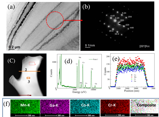
FIG. 6. (a) TEM image (thickness fringes running over the image) (b) Selected area electron diffraction (c) Scanning TEM-HAADF image (d) Energy dispersive X-ray (EDX) spectrum from point 1 (e) EDX line-profile from line 2 in (c) (f) Elemental mapping from area 3 in (c).
