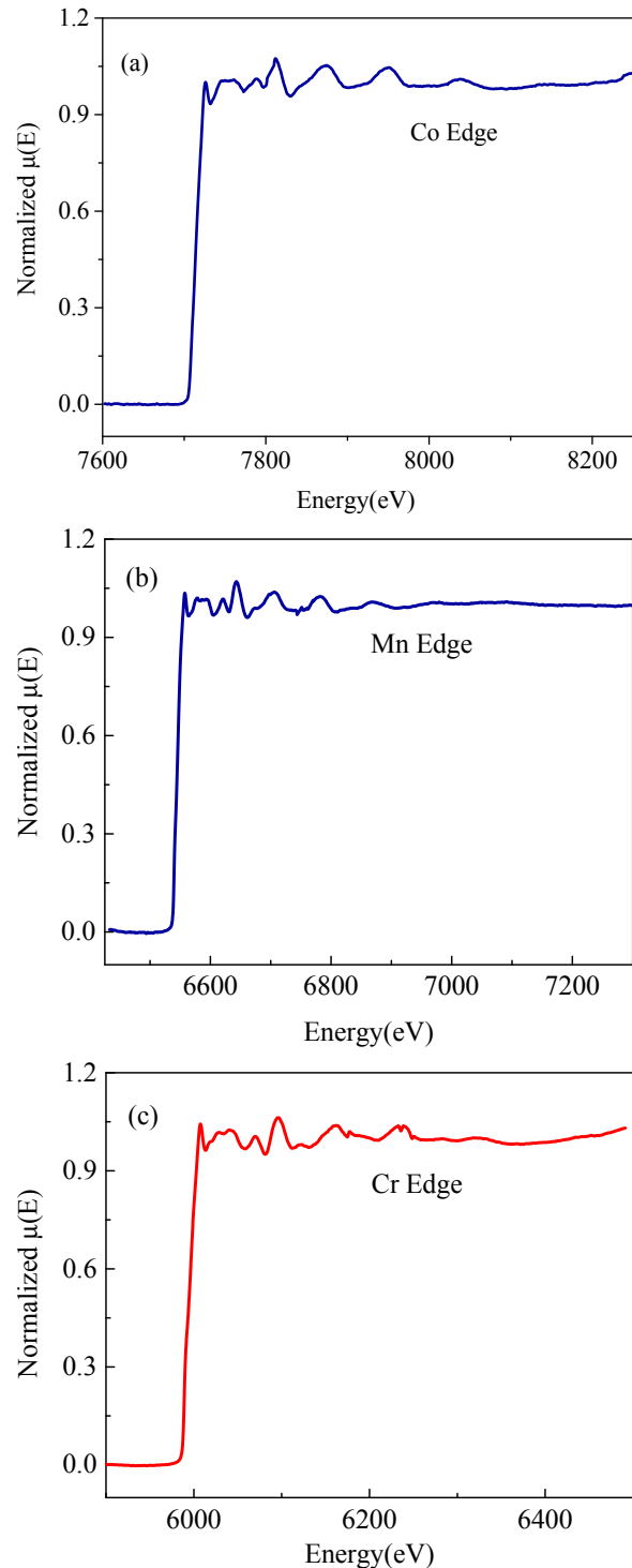
FIG. 7. Normalized EXAFS spectra of \text{CoMnCrGa} taken at (a) Co edge (b) Mn edge and (c) Cr edge.
