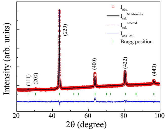
FIG. 5. Rietveld refinement of the powder XRD pattern of CoMnCrGa assuming disordered structure & ordered structure measured at room temperature. The two fits got overlapped and remain essentially indistinguishable. Bragg peaks are mentioned in vertical first bracket.
