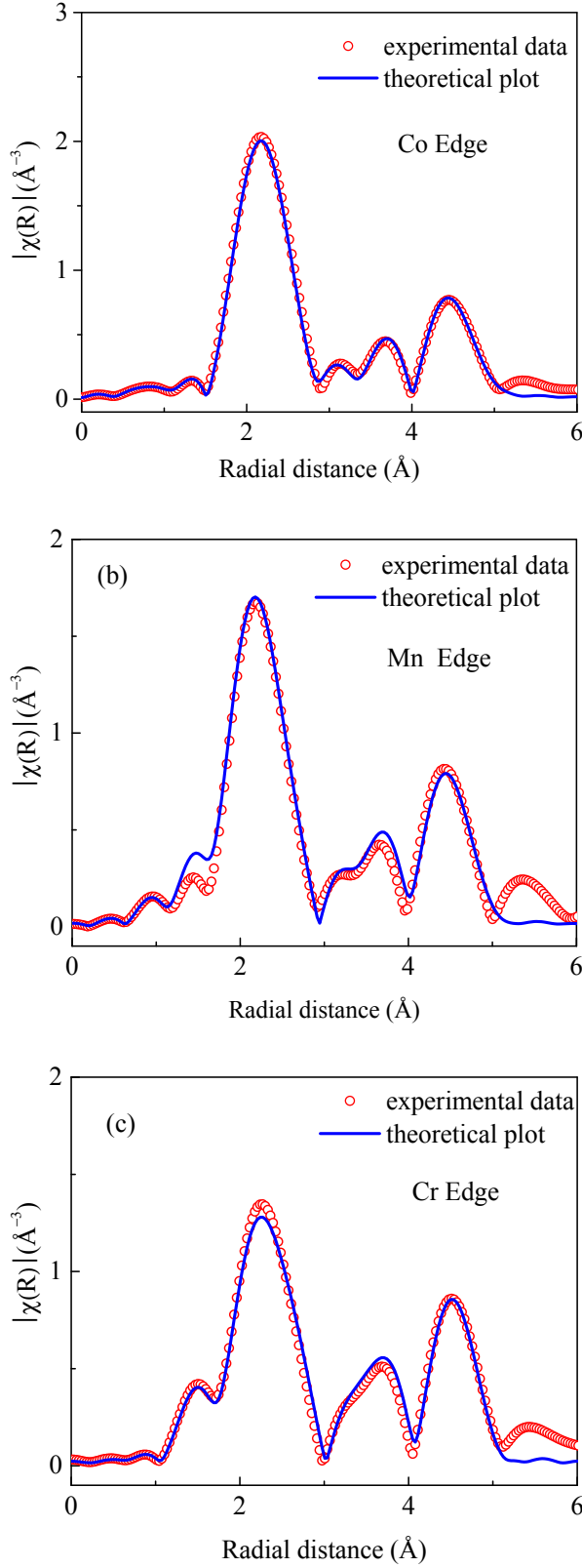
FIG. 8. Fourier transformed EXAFS spectra of CoMnCrGa taken at Co, Mn and Cr edges.
