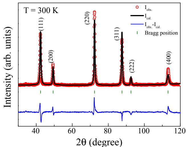
FIG. 3. Rietveld refinement of the neutron diffraction pattern (taken at 300 K) of CoMnCrGa, considering the crystal structure only.
