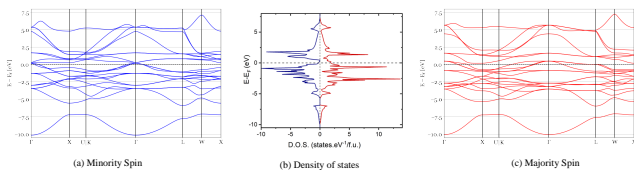
FIG. 1. Spin-polarized band structure and density of states of CoMnCrGa in ordered Type 2 structure: (a) minority spin band (b) density of states, (c) majority spin band.
