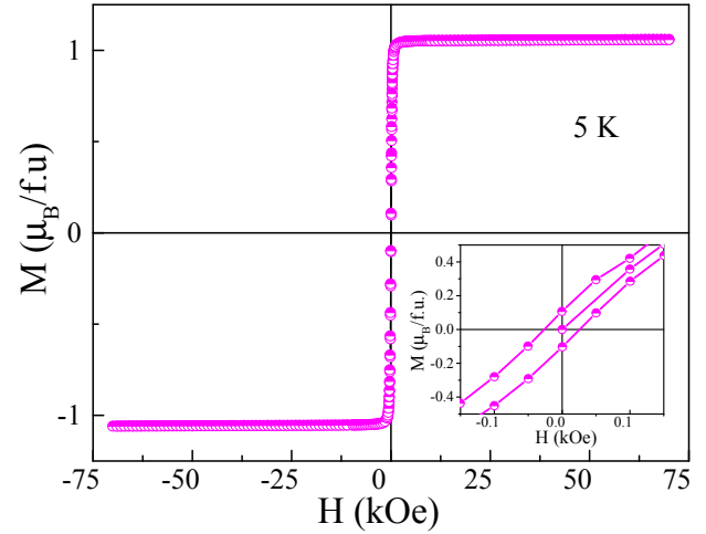
FIG. 10. Isothermal magnetization of CoMnCrGa measured at 5 K. Inset shows the enlarged view of coercivity in low field region.
