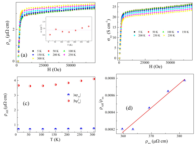
FIG. 12. (a) Field-dependent Hall resistivity curves at different temperatures. Inset shows temperature variations of carrier concentration (b) Field-dependent Hall conductivity curves at different temperatures. (c) Different contributions in \rho_{AH} with temperature are plotted on the same scale. (d) Fitting of the ratio of anomalous Hall resistivity and longitudinal resistivity.
