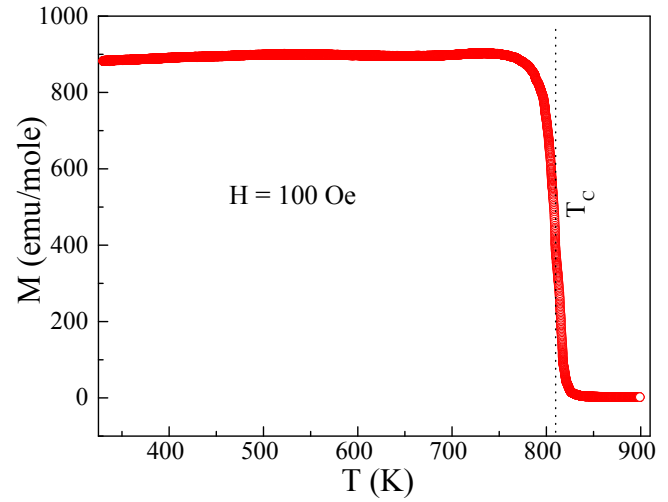
FIG. 9. Temperature dependence of magnetic susceptibility of CoMnCrGa measured in a 100 Oe applied magnetic field. Curie temperature, T_C , is determined from the minima in dM/dT vs. T plot.
