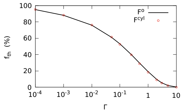
FIG. 4: Theoretical transmitted fraction f_{\text{th}} (in percentage) as a function of the dimensionless parameter \Gamma defined by Eq. 9 in the case of a uniform, divergence-less ion beam aligned with the capillary axis. Full black line has been computed using F_{\text{im}}^{\circ} while the red circles were obtained with F_{\text{im}}^{\text{cyl}} = F_{\text{im}}^{\circ} \times h_{\epsilon_r} and \epsilon_r = 2 .
