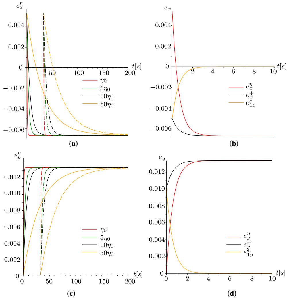
Fig. 14 Evolution and redistribution of viscous and elastic strains: a, c evolution of viscous strains e_x^\eta and e_y^\eta , respectively, in the point \zeta = 0 from the moment t = 0 and in the point y front the moment t_y = 30 s for various viscosity coefficients; b, d redistribution of elastic strains e_{1x}^e , e_{1y}^e and viscous strains e_x^\eta , e_y^\eta within total strains e_x^+ , e_y^+ in the point \zeta = 0 . Solid and dashed lines of the same color correspond to the same viscosity
