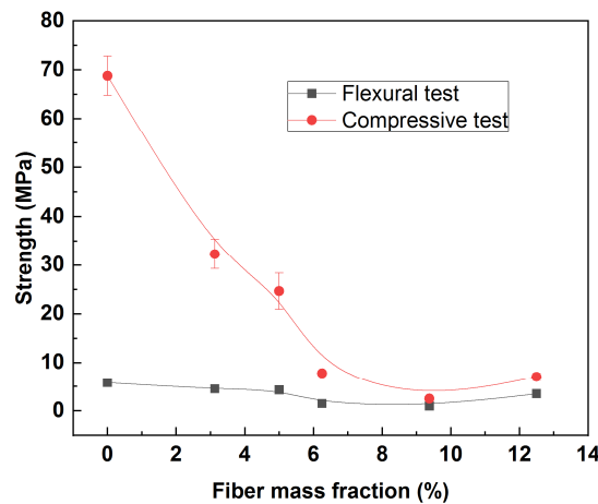
Figure 10 : Evolution of flexural and compressive strengths as a function of fiber mass fraction.
