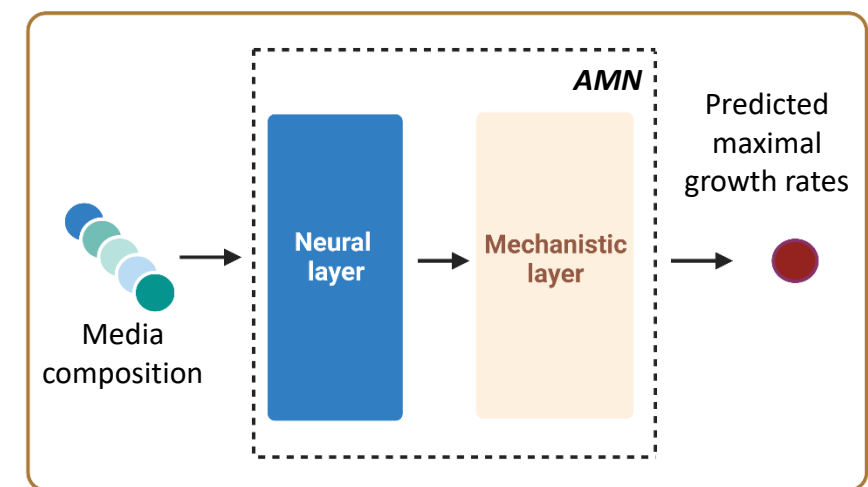
AMN training
