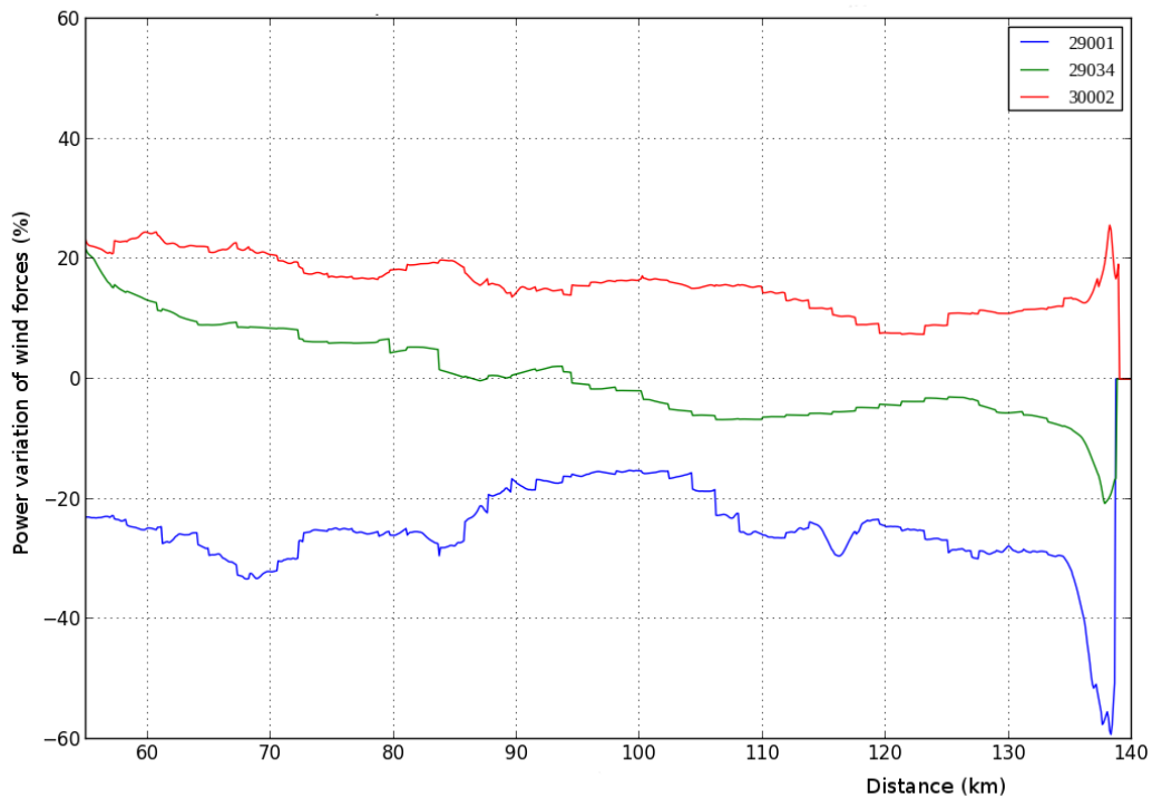
Fig. 6. Power variation of wind forces for three particular test runs (labelled 29001, 29034 and 30002).
