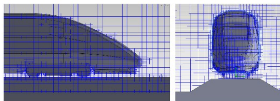
Fig. 3. Transverse and frontal views of the numerical discretization of the train.
