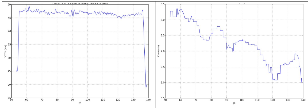
Fig. 5. Train speed (left) and computed wind speed (right) for the 30002 test run along the curvilinear distance pk (km)
