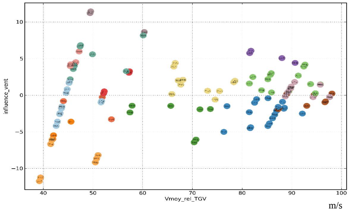
Fig. 2. Classification of the runs on the train speed, and relative wind speed (each colored spot represent a test run).
