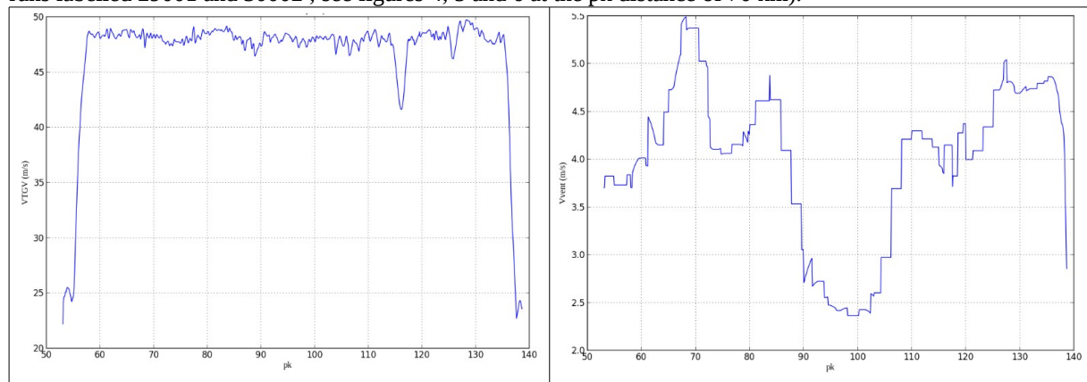
Fig. 4. Train speed (left) and computed wind speed (right) for the 29001 test run along the curvilinear distance pk (km)
