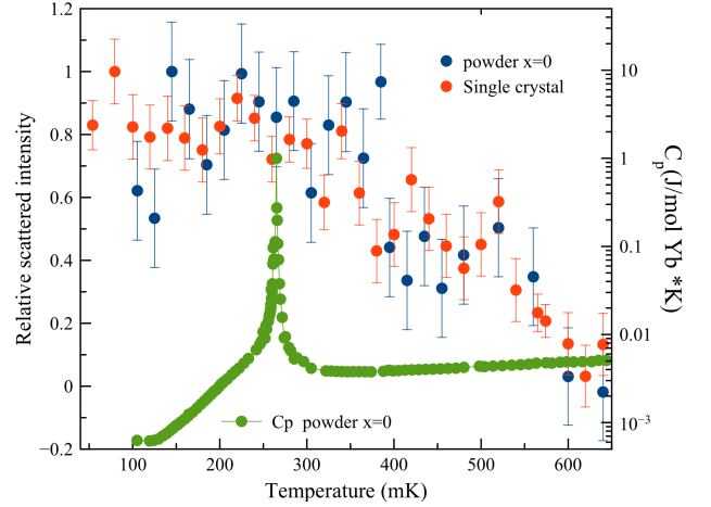
FIG. 3: The temperature dependence of the elastic scattered intensity at |\vec{Q}|=(111) . – The scattered elastic neutron intensity, relative to T=700 mK at |\vec{Q}|=(111) shows similar temperature dependence for both a previously measured single crystal (data taken from Ross et al. 14 ) and for the stoichiometric powder sample of \text{Yb}_2\text{Ti}_2\text{O}_7 (this work). With increasing temperature, the elastic magnetic scattering begins to fall around T = 0.35 K, and decreases approximately linearly above this temperature. The specific heat anomaly T_C \sim 0.26 K for a representative powder sample of \text{Yb}_2\text{Ti}_2\text{O}_7 (data taken from ref Ross et al. 28 ) is shown for reference, and reveals the relative insensitivity of the temperature dependence of the elastic scattering to the specific heat anomaly.
