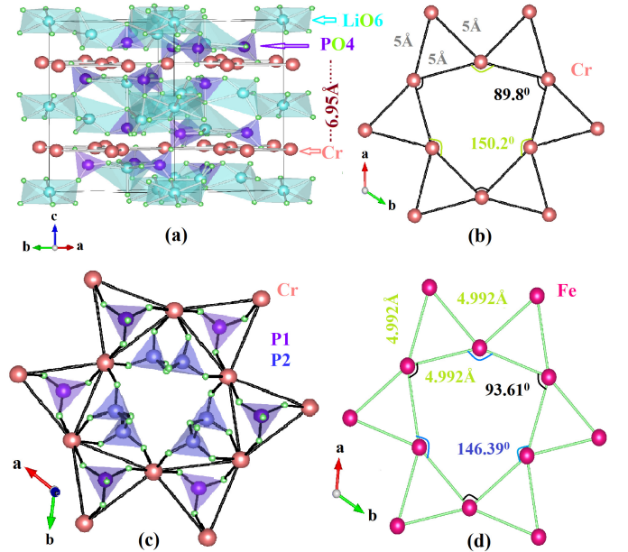
Figure 2: The crystal structure of LCPO drawn using VESTA program [48]. (a) A representative unit-cell of LCPO with kagomé layers (Cr) separated by LiO 6 octahedra (light cyan) and PO 4 tetrahedra (light violet). (b) A view of kagomé plane formed by Cr - atoms in ab - plane. (c) Interaction pathways between Cr - atoms, for a kagomé motif, mediated through PO 4 bridges. (d) A view of kagomé plane formed by Fe - atoms (in LFPO) in ab - plane. (Note: P1 (violet) is located apically the center of each triangle and its position changes alternatively from z to -z on moving from one to the next triangle, while P2 (light blue) is structurally positioned in the kagomé hexagon)
