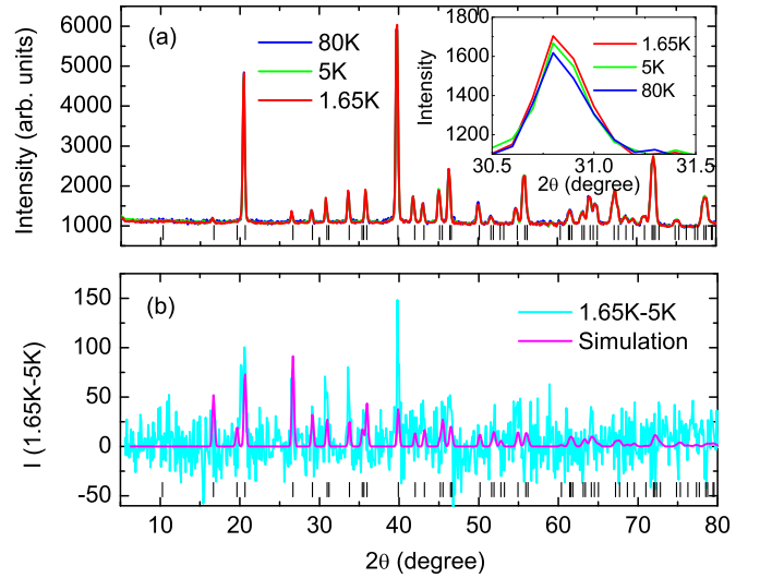
Figure 4: (a) Neutron diffraction profiles measured at T = 80, 5, and 1.65 K. Inset depicts the zoomed portion of diffraction profile around the Bragg position \sim 30.8^\circ . (b) Difference profile (cyan line) after subtracting out the 5 K data from the 1.65 K data. The pink solid line represents a simulated pattern for a ferromagnetic model with k = 0 and ordered moment 1.05 \mu_B . The negative intensity in the vicinity of some of the Bragg positions results due to a noisy background.
