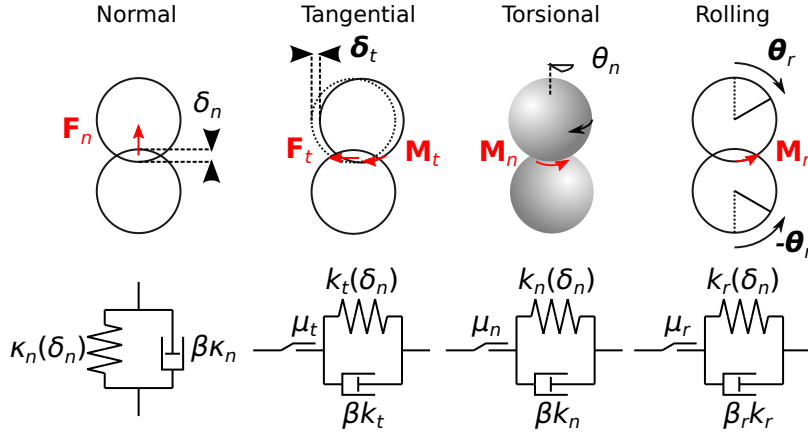
Figure 1. Schematic of simulations' interparticle interactions. Between two particles in contact, the simulated normal and tangential forces ( \mathbf{F}_n and \mathbf{F}_t ) and couples ( \mathbf{M}_n , \mathbf{M}_t , and \mathbf{M}_r ) depend on the particles' normal and tangential deformations ( \delta_n and \delta_t ) and angular deformations ( \theta_n and \theta_r ). Behavior is viscoelastic and, except in the case of the normal reaction force, friction-limited, so interactions can be modeled at each timestep by the systems of springs, dashpots, and friction elements that we represent below each force diagram, with viscosities \beta\kappa_n , \beta k_t , \beta k_n , and \beta_r k_r proportional to the \delta_n -dependent spring stiffnesses \kappa_n , k_t , k_n , and k_r , and friction coefficients \mu_t , \mu_n , and \mu_r .
