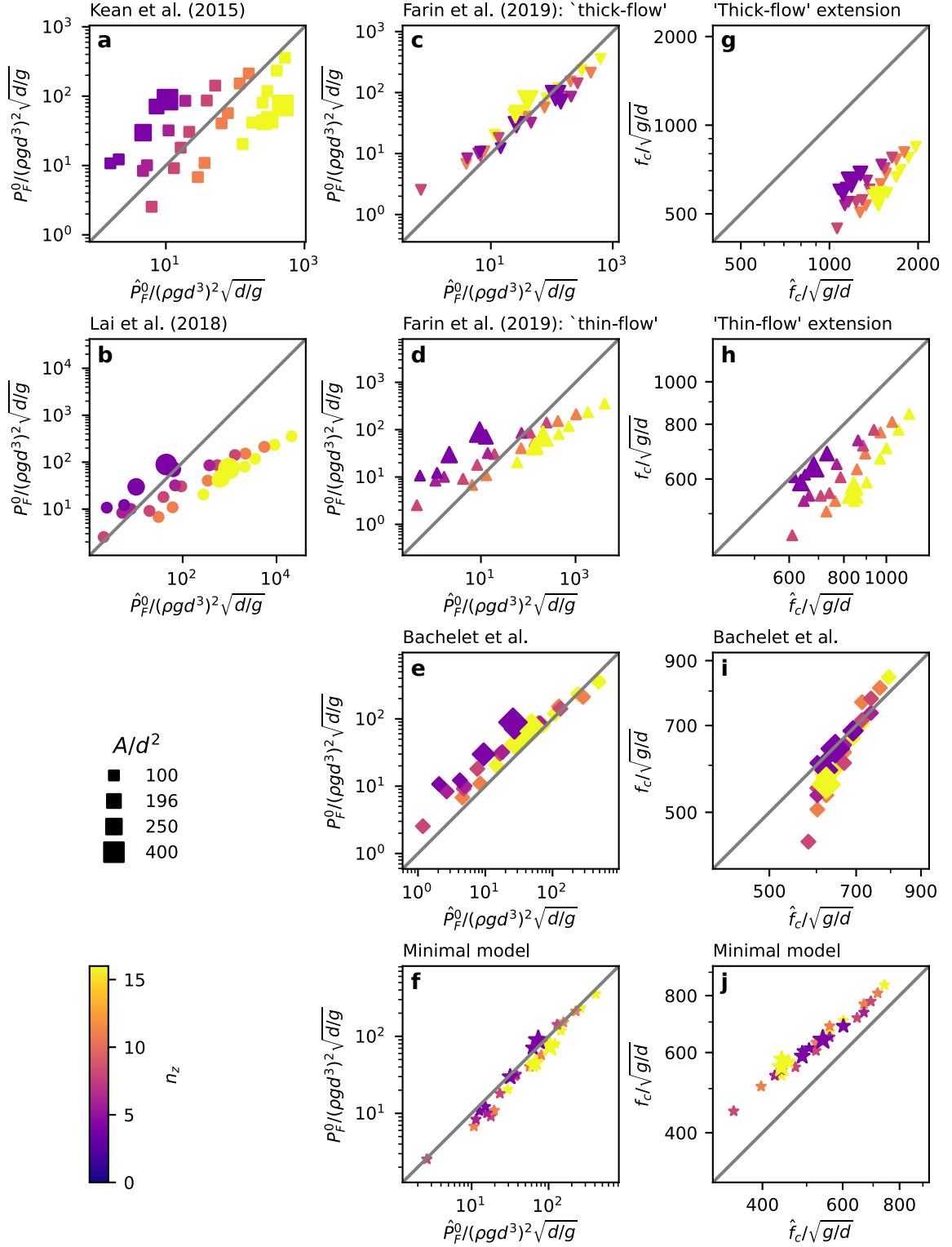
Figure 5. Comparison between models' predictions ( x -axes) and simulation outputs ( y -axes) for the low-frequency amplitudes (a-f) and corner frequencies (g-j) of high-frequency signals. The gray lines represent perfect agreement, while marker size indicates measurement area A (with A/d^2 = 250 for channel flows) and colors indicate flow overburden n_z . For each n_z , P_F^0 and f_c increase with \theta .
