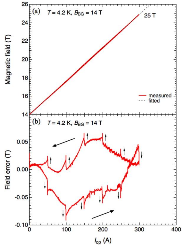
Fig. 3. (a) Generated magnetic field measured by a Hall probe at the center of 20-stacked coils under a background field of 14 T. (b) Difference between the measured value and the fitted line as a function of the operating current.
