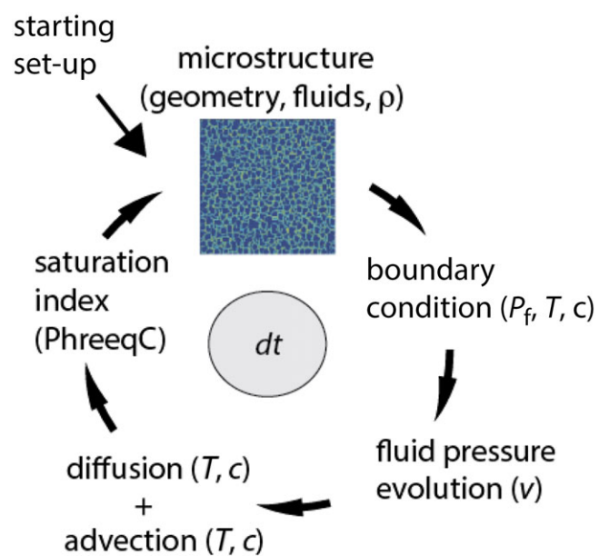
Fig. 2. Schematic diagram illustrating the simulation model set-up. An initial structure with certain starting conditions builds the base of the system with a background porosity, temperature, fluid pressure and pore fluid with concentration of species and density. The model then applies boundary conditions fluid pressure ( P_f ), temperature ( T ) and concentration of different species of the incoming fluid ( c ). The next step in the model is the evaluation of the fluid pressure evolution per time step followed by transport of temperature and concentration by advection and diffusion. The local concentration of species and temperature are then used in iphreeqc to calculate the local fluid properties including density and saturation indices of minerals.
