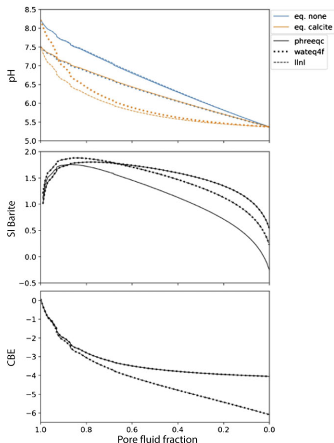
Fig. 4. Ideal mixing of pore fluid (seawater) and infiltrating fluid (oil-field brine) calculated using MIX in the iphreeqc module. pH, barite saturation state and CBE are obtained for three databases: phreeqc (solid lines), wateq4f (dotted lines) and lnl (dashed lines). The blue lines represent the mixing with unaltered seawater and the orange lines show the resulting fluid if mixed with seawater equilibrated with calcite. Equilibration with quartz did not alter the results compared with the non-equilibrated case; only the experiments with non-equilibrated and calcite-equilibrated pore fluid are shown.
