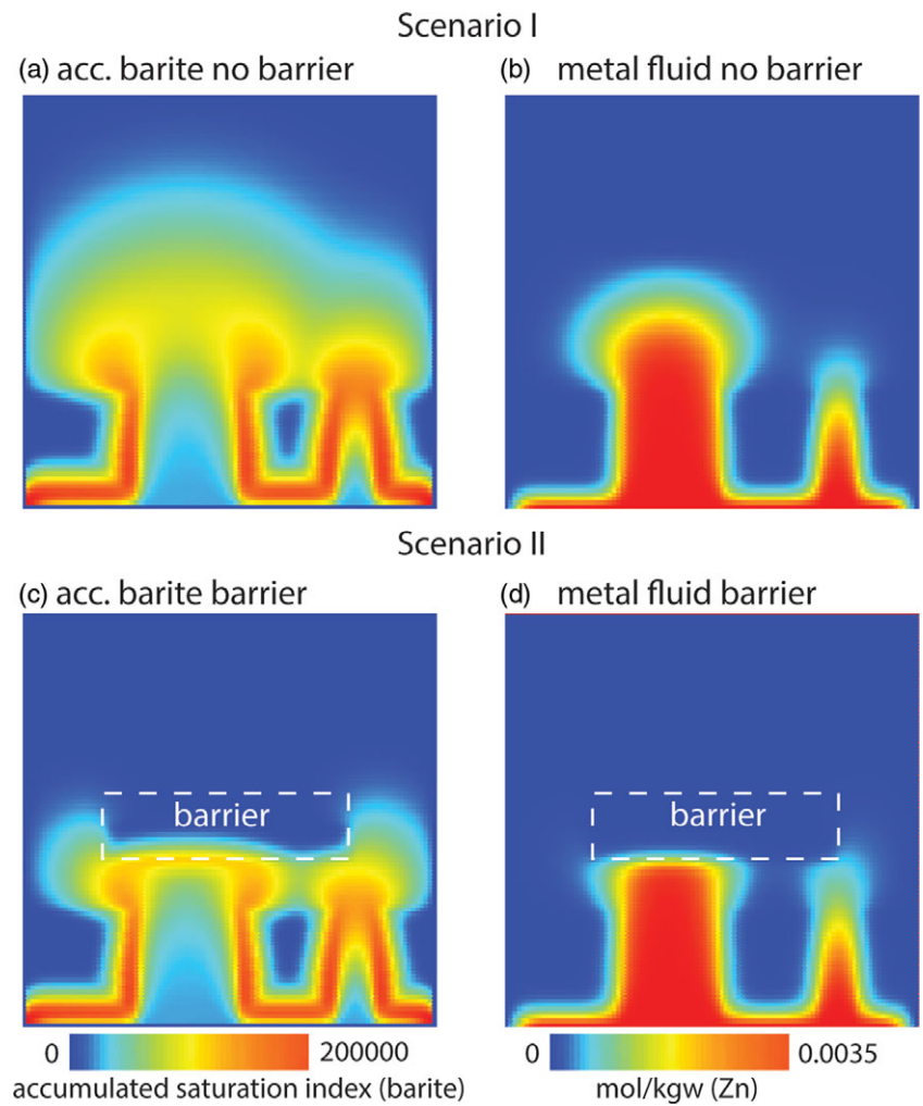
Fig. 8. Effects of horizontal permeable layer and a horizontal low-permeability layer on flux and saturation index of barite. (a) Accumulated barite saturation index in a simulation with a permeable layer on top of the two faults but no seal. High saturation index above the fault is present on the fault sides and where fluids between the two faults mix as a result of diffusion. (b) Concentration of incoming metal fluid for scenario I. (c) Accumulated barite saturation index in a simulation with a horizontal permeable layer covered by a central low-permeability layer (scenario II). (d) Concentration of metal fluid in scenario II. Fluid is pushed against the barrier and flows around it at the left- and right-hand side. Below the barrier the accumulated saturation index of barite is high, indicating that barite would precipitate at this location. All pictures shown are after 115 days.
