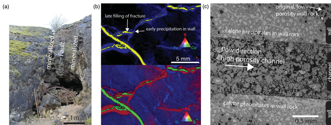
Fig. 1. Example of mineralization at different scales within and adjacent to high-permeability sites. (a) Mineralization associated with faulting, Trollers Gill Barite-Fluorspar-Galena mine, Yorkshire Dales, UK. (b) MicroXRF geochemical mapping image acquired with a Bruker M4 Tornado from the hole NDIBK04 drilled by the National Drilling Initiative through the MinEx CRC. NDIBK04 is the most prospective well in the East Tennant Creek (Northern Territory) NDI region, an emerging mineral province for base metal mineral exploration (Zn, Cu and As). This sample is from the top of a c. 150-m-thick banded graphitic schist of the Palaeoproterozoic Alroy Formation intersected at depth 236.2–237 m. The nearest geochronology available is from a sample at 301–307 m depth, giving a maximum depositional age of 1969 \pm 10 Ma (dated by SHRIMP at Geoscience Australia with zircons). The main vein has gypsum at its centre with Fe–Mn-rich carbonate to the edge. Such vein geometries can arise from the interaction with different fluids or by the evolution of a single infiltrating fluid with the host rock. The presence of gypsum in the centre of the vein points towards an open channel that prevailed after the diffusion-dominated reaction between fluid and rock that led to the development of the reaction rims surrounding the veins. (c) Experiment of calcite precipitation in low-porosity dolomite directly adjacent to high-porosity fracture in response to carbonate-rich fluid infiltration (courtesy of R. Morgan and Q. Fisher).
