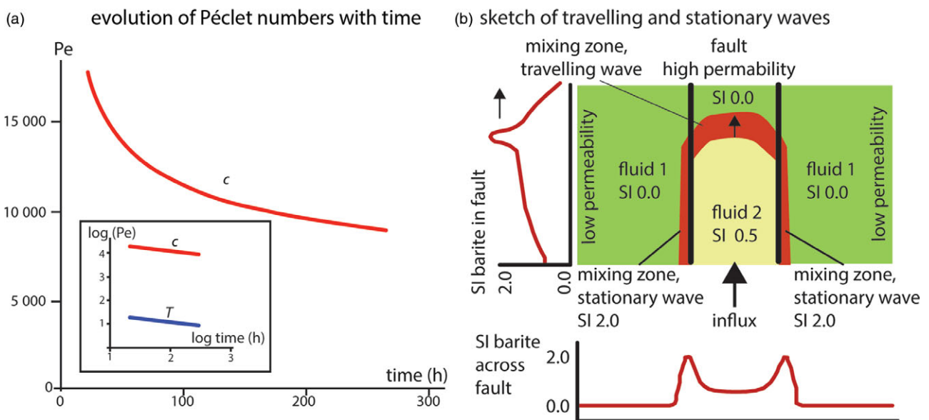
Fig. 10. (a) Initial evolution of the Péclet number ( Pe ) with time in the simulations. Initially, the Péclet number for concentration of species is decaying fast. Inset shows a log-log plot of Péclet numbers for concentration versus temperature, illustrating that temperature is a lot more diffusion controlled than concentration. (b) Schematic illustration of a high-permeability fluid channel or fault with a travelling wave of high saturation index of barite. Stable waves develop in the wall rock of the fault where mineralization can occur. A plot of SI barite along the fault on the left-hand side of the figure shows a snapshot of the travelling wave of high-SI barite, whereas the plot at the bottom of the figure shows the stationary waves of high-SI barite in the wall rock of the faults. The index is only high where the mixing between the fluids is optimal, with c . 80–90% of pore fluid and only a small amount of incoming fluid of 10–20%. The index therefore decays once the incoming fluid dominates and displaces the pore fluid. The geometries are similar to the experiment shown in Figure 1c, even though the experiment did not directly involve fluid mixing.
