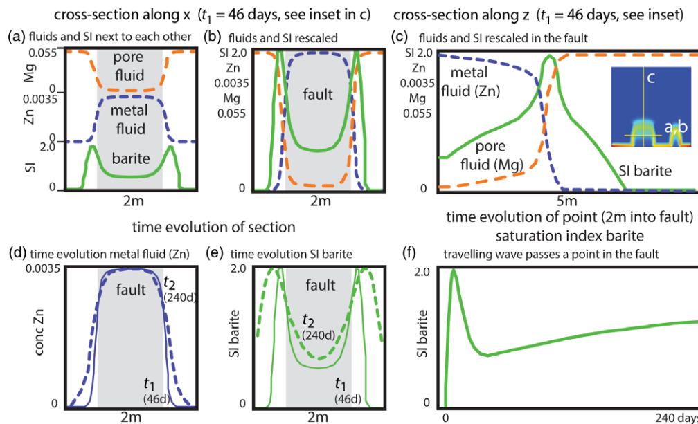
Fig. 6. Evolution of pore fluid, metal fluid and barite saturation index in one fault. (a, b) Cross-section through a fault where the metal fluid has infiltrated: (a) fluids and barite solution index in three plots and (b) all confined to one plot; mixing best in the fault walls. (c) Vertical section through the incoming metal fluid showing how the pore fluid is pushed away and the barite saturation index is highest within the area where 80% of pore fluid is still present. This wave of high barite saturation index is moving with the infiltrating fluid through the fault. (d) Two evolutions for the incoming fluid where the concentration curve flattens out into the wall rock as a result of diffusion. (e) Saturation index of barite for (d), showing how the maxima move with diffusion into the wall rock of the fault. (f) Time evolution of a point in the model with a very fast increase in barite saturation index when the fluids mix, followed by a relaxation when the metal fluid dominates (full model run is 231 days).
