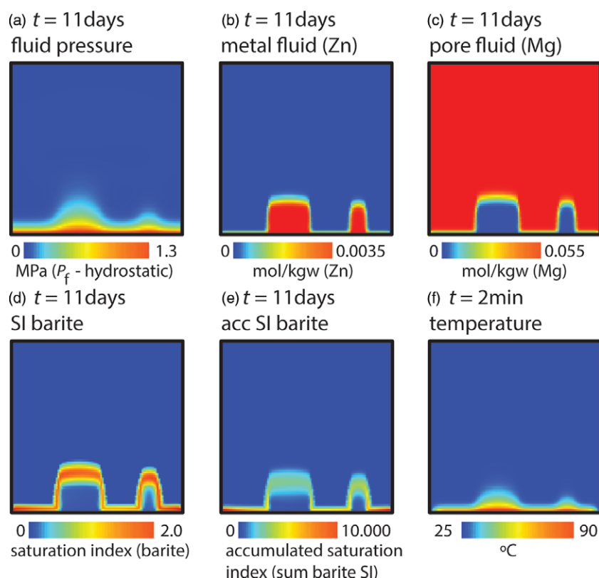
Fig. 5. Evolution of fluid in two vertical faults with blue low and red high numbers; width of box is 5 m. (a) Evolution of the fluid pressure into the two faults. (b) Influx of metal-rich fluid into the faults with a Péclet number (see Section 4b for definition) of around 8000 for concentration in the fault. (c) Pore-fluid is displaced in the faults by the incoming fluid. (d) Evolution of barite saturation index in the faults. (e) Barite saturation index summed up over time to show how long the saturation index is high. (f) Temperature after 2 min of model run. Temperature is equilibrating as a result of fast diffusion (T-Péclet number of 100 at the start, and 8.3 after 11 days in the fault).
