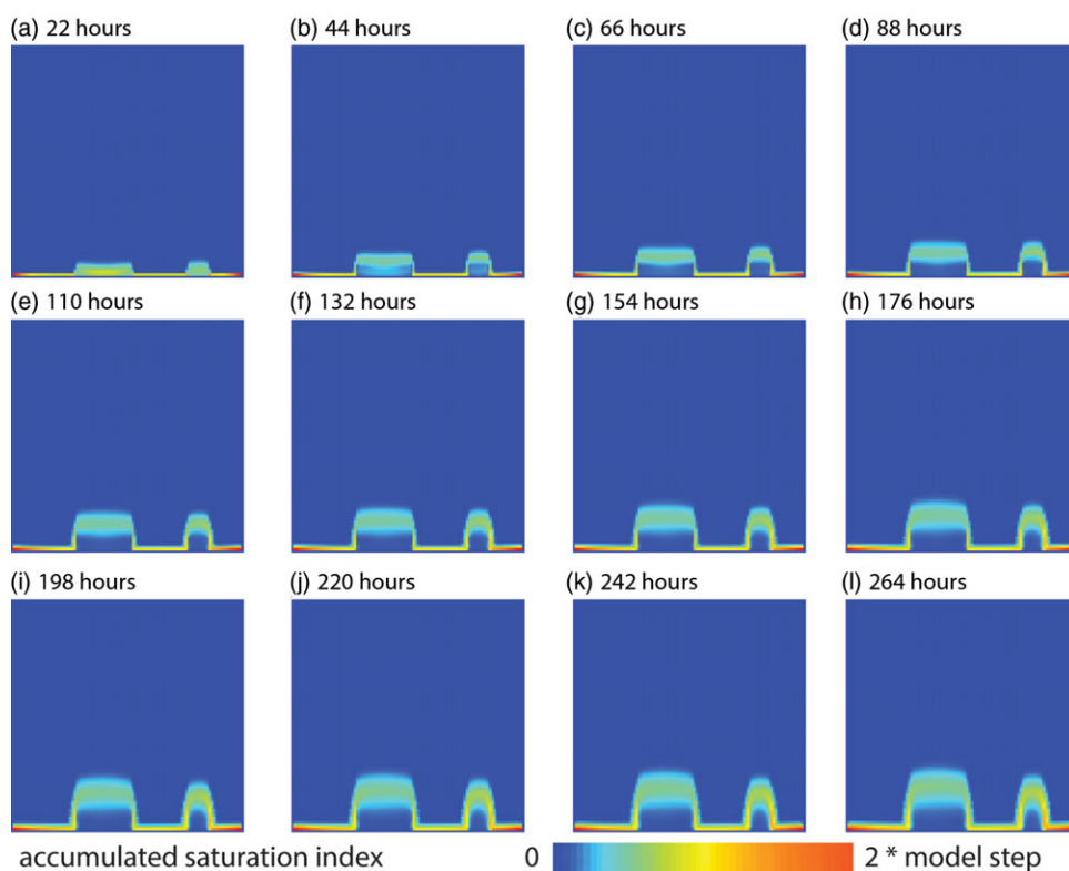
Fig. 7. Evolution of summed saturation index of barite in the faults: (a–l) progressive time steps. The saturation index shows a relatively stationary and diffusion-controlled wave of high accumulated SI of barite in the wall rock, but a travelling wave of high SI of barite in the faults that grow in width.
