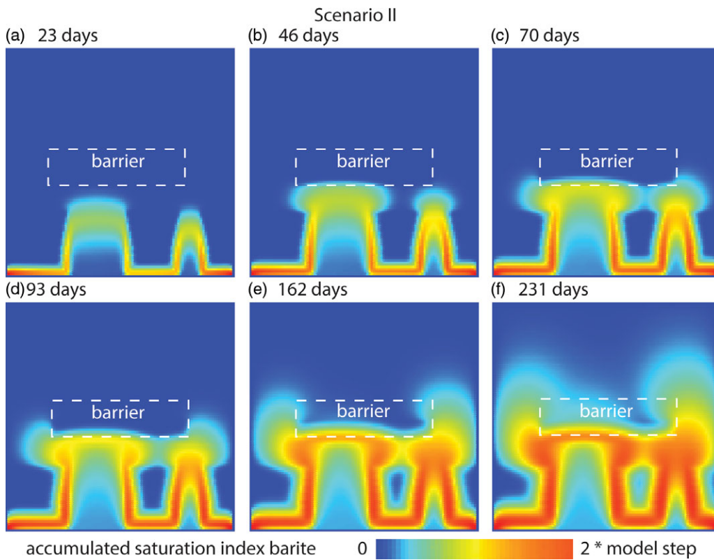
Fig. 9. Time evolution of the accumulated saturation index of barite in simulations with a permeable layer and a barrier (scenario II). The highest indices are in the fault walls, between and at the exit of faults, in the permeable layer and below the barrier.
