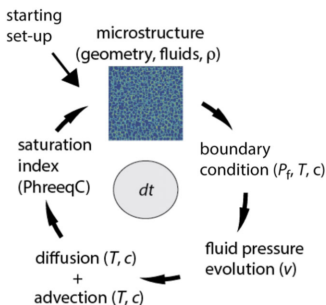
Fig. 2. Schematic diagram illustrating the simulation model set-up. An initial structure with certain starting conditions builds the base of the system with a background porosity, temperature, fluid pressure and pore fluid with concentration of species and density. The model then applies boundary conditions fluid pressure ( P_f ), temperature ( T ) and concentration of different species of the incoming fluid ( c ). The next step in the model is the evaluation of the fluid pressure evolution per time step followed by transport of temperature and concentration by advection and diffusion. The local concentration of species and temperature are then used in iphreeqc to calculate the local fluid properties including density and saturation indices of minerals.
