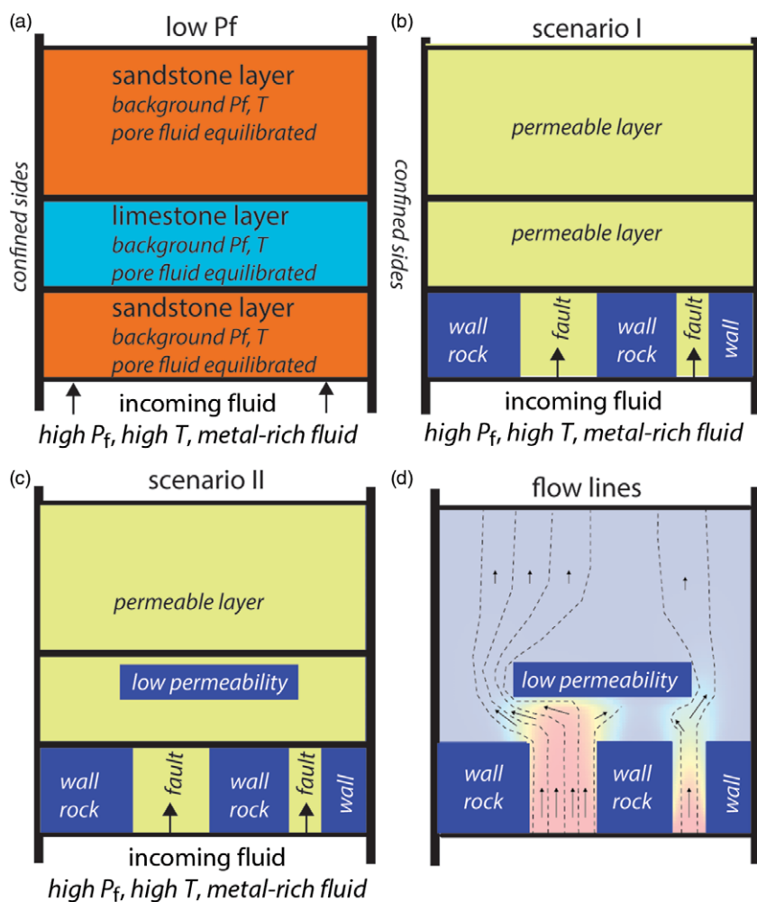
Fig. 3. Set-up of the simulations. (a) Mineralogy of the layers with two sandstone layers and one limestone layer in the centre. Initial boundary conditions are defined by equilibrated pore fluid in the different layers. Side walls are confined so that no fluid escapes sideways. The upper boundary is open and contains a low fluid pressure. The metal fluid enters through the lower boundary with an initially increasing and then constant fluid pressure, temperature and incoming fluid composition at the lower boundary. (b) Porosity/permeability scenario I with two permeable faults in the otherwise low-permeability lower layer. (c) Porosity/permeability scenario II with an additional low-permeability horizontally aligned area in the centre of the model above the two faults. (d) Flow lines for scenario II showing how flow concentrates in the two faults and then spreads out in the high-permeability layers and goes around the low-permeability zone in the centre.
