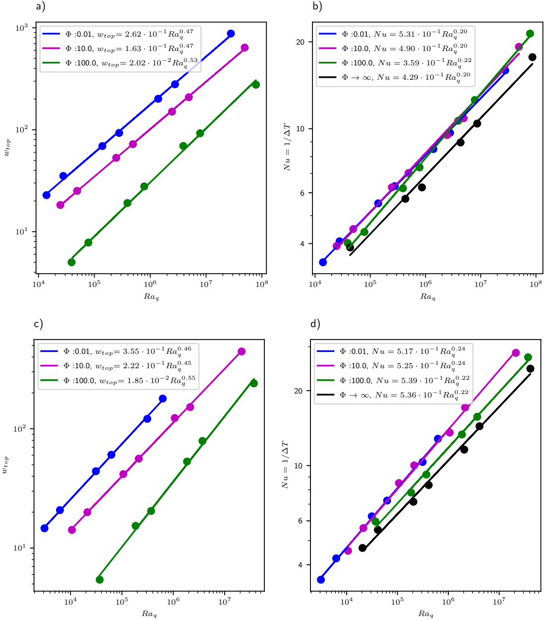
Figure 8: Cases Ra_q \geq 50Ra_c for a rigid bottom BC (a)&(b) and a free-slip bottom BC (c)&(d). Left panels (a)&(c) show the dimensionless radial velocity at the top boundary of the HP ice layer. Right panels (b)&(d) show the dimensionless heat flux (Nusselt number). Both parameters in function of the Rayleigh Number and for various values of \Phi .
