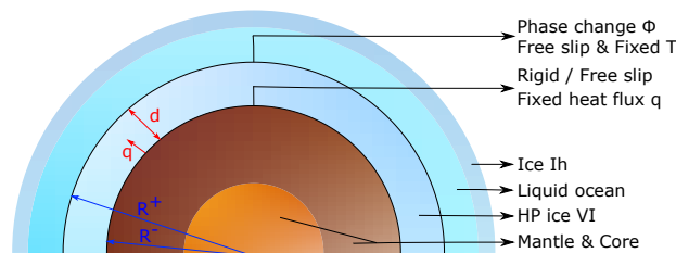
Figure 1: Model illustration for the interior of an ocean world with an HP ice layer in direct contact with a liquid ocean at top and a rocky core/mantle at the bottom (type IV or V of Lammer, 2013, and type H3 of Noack et al., 2016). Our numerical models treat convection in the HP ice layer.
