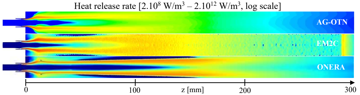
Figure 16: Case OM-5kHz. Longitudinal slices of mean heat release rate ( y - z plane).
