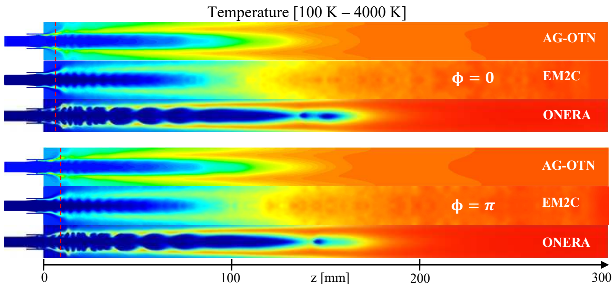
Figure 18: Case OM-5kHz. Longitudinal slices of phase-averaged temperature ( y - z plane) for two distinct phases.
