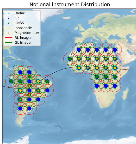
Figure 2: Notional distribution of instruments on the South American and African continents. Additional instrumentation would be deployed to cover ocean regions.
