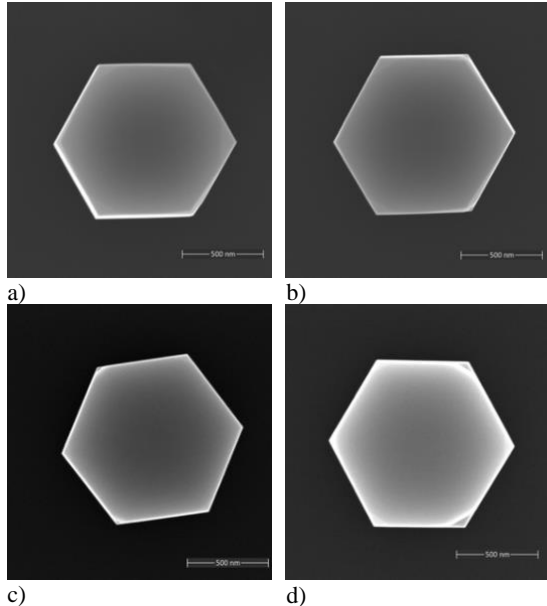
Figure 2: Top SEM images of \mu -scale GaAs crystal sgrown on silicon using the ELTO Process for different V/III ratio with TBAs and TEGa as gas precursors. a) R = 6 , b) R = 10 , c) R = 18 and d) R = 22 .
