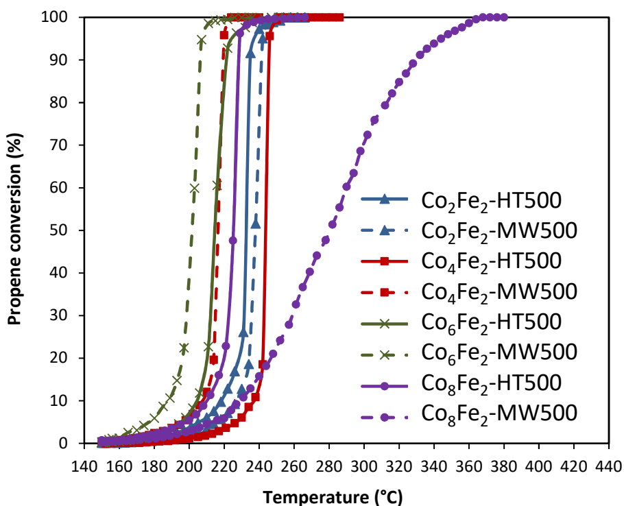
Fig. 3. Propene conversion to \text{CO}_2 versus reaction temperature on \text{Co}_x\text{Fe}_2 -HT500 and \text{Co}_x\text{Fe}_2 -MW500 samples
