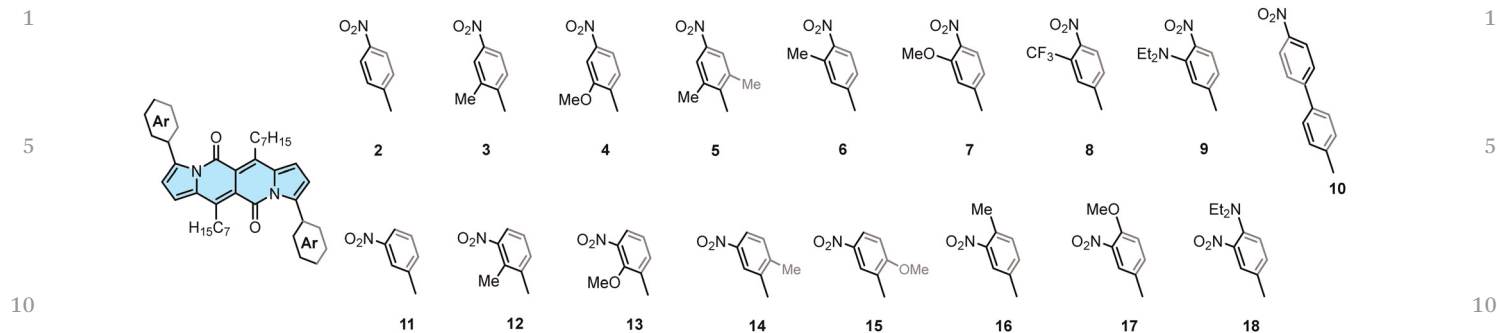
Fig. 2 Structure of nitroaromatics studied in this work.
