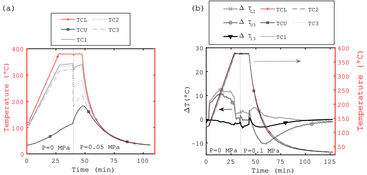
Figure 3: Thermocouple measurements during one-sided heating with natural cooling (a) and two-sided heating with enforced cooling (b) cycle of deconsolidation experiments. On the right graph (b) the temperature is much more homogeneous. Temperature differences are plotted along the left axis. We can see the thermal effect of pressure application during dwell.
