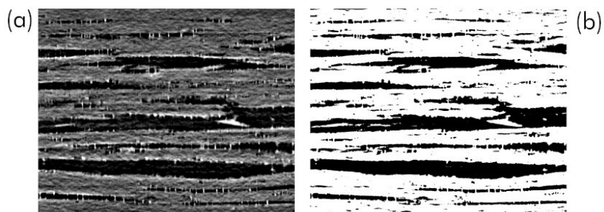
Figure 5: Comparison between a grey scale (a) and segmented (b) slice parallel to the fibers' orientation, through the thickness of a deconsolidated laminate. The black zones represent the pores.
