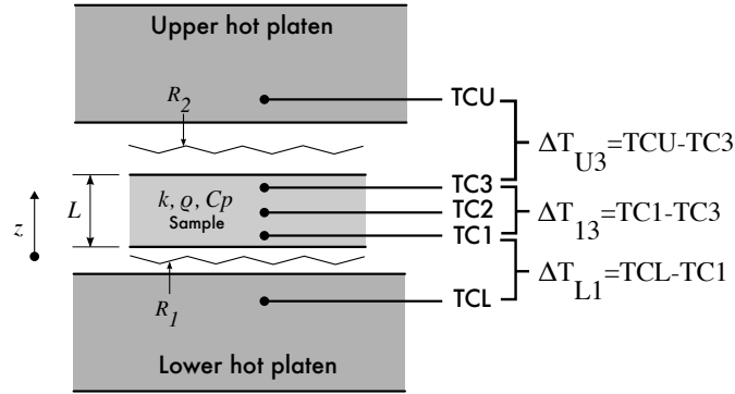
Figure 2: Estimation of the effective laminate temperature using a through thickness 1D heat transfer model. The model is fitted using 5 thermocouple measurements. R_1 and R_2 represent the thermal resistances between (i) the lower hot platen and composite lower face and (ii) the composite upper face and the upper hot platen.
