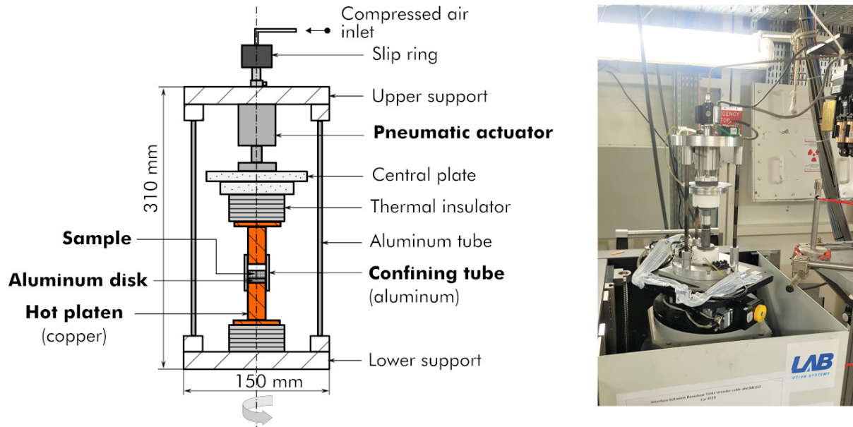
Figure 1: In situ Composite Deconsolidation Tomography Observation setup. Schematic view (left) and picture of the device installed onto the rotation stage of the ID19 beamline X-Ray microtomograph (right).
