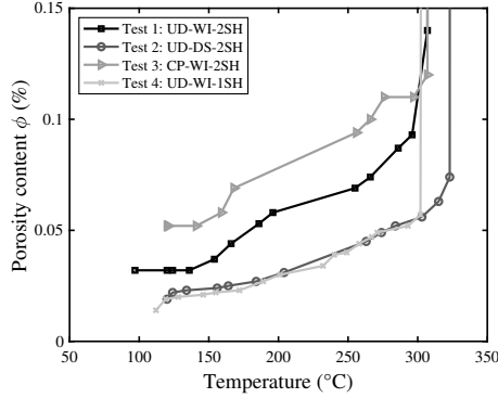
Figure 10: Zoom of the previous figure showing the porosity \phi as a function temperature estimated with the thermal model during the deconsolidation tests. The dashed circles indicate the onset temperature of deconsolidation.
