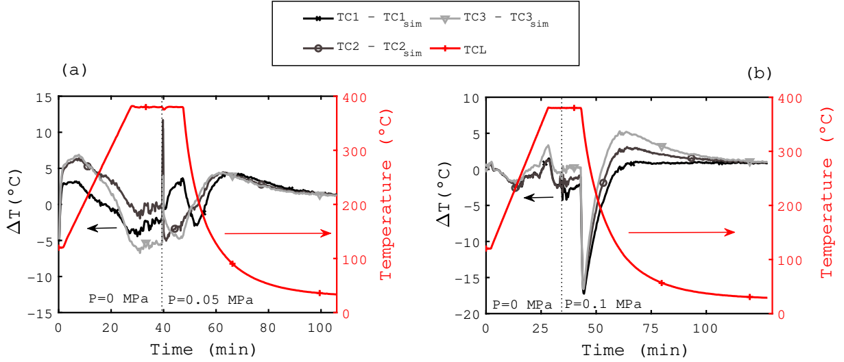
Figure A.17: Thermal model validation for the two heatings at different pressures: one-sided heating with NAP + P=0.05 MPa (a) and two-sided heating with NAP + P=0.1 MPa (b).
