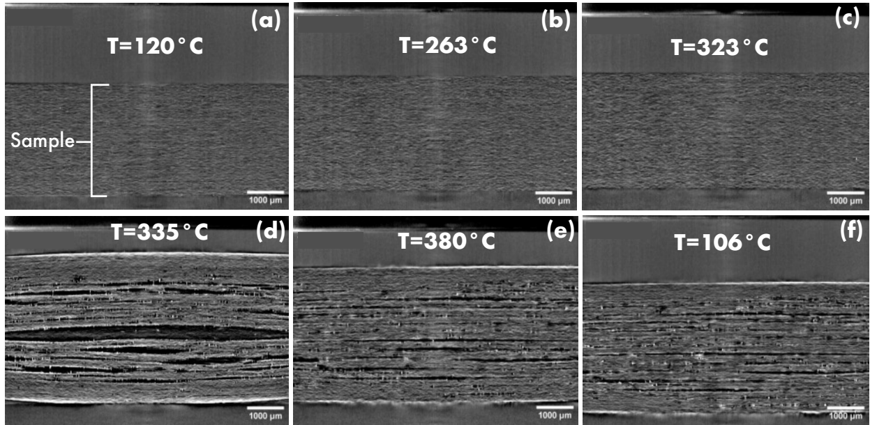
Figure 6: Tomographic cross section evolution over a temperature cycle of an initially dried [UD]_{16} composite sample for 72h@180°C (UD-DS-2SH). The black spots represent the pores.
