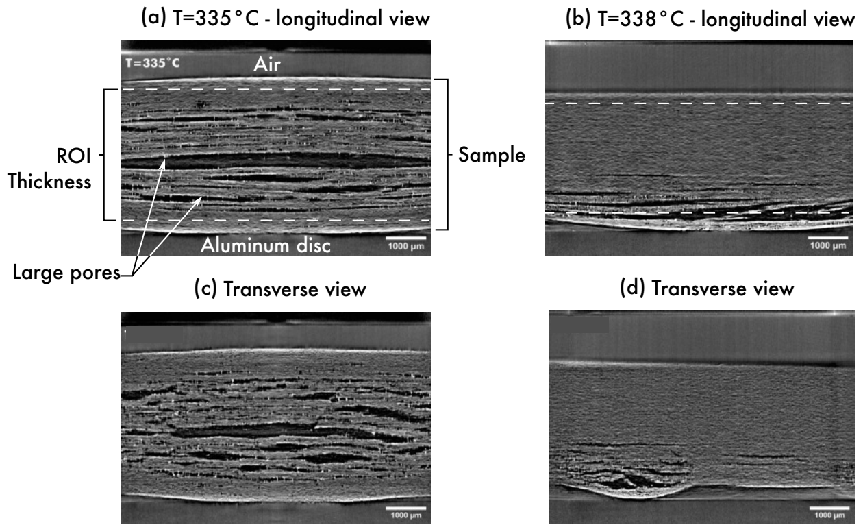
Figure 4: 2D grey level slices through the thickness of a deconsolidated UD laminate showing the ROI thickness and pore during two-sided heating (a,c) and one-sided heating (b,d). The slices are parallel to the fibers' orientation in (a,b) and transverse to the fibers in (c,d).
