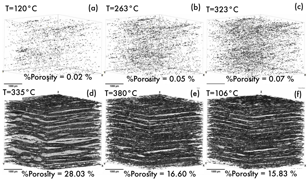
Figure 7: Time evolution of the porosity in a ROI of 3.81 \text{ mm} \times 3.81 \text{ mm} \times Z during deconsolidation of an initially dried [\text{UD}]_{16} composite sample for 72\text{h}@180^\circ\text{C} . The axis (OX) and (OY) are respectively parallel and transverse to the fibers' main axis. The black spots represent the pores.
