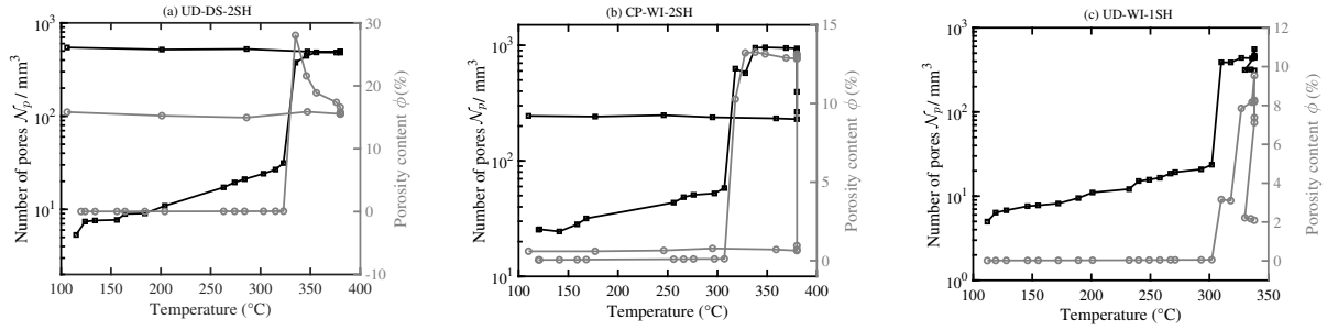
Figure 12: Evolutions in pore density \mathcal{N}_p and porosity \phi with the temperature during deconsolidation experiments: UD-DS-2SH (a), CP-WI-2SH (b) and UD-WI-1SH (c).
