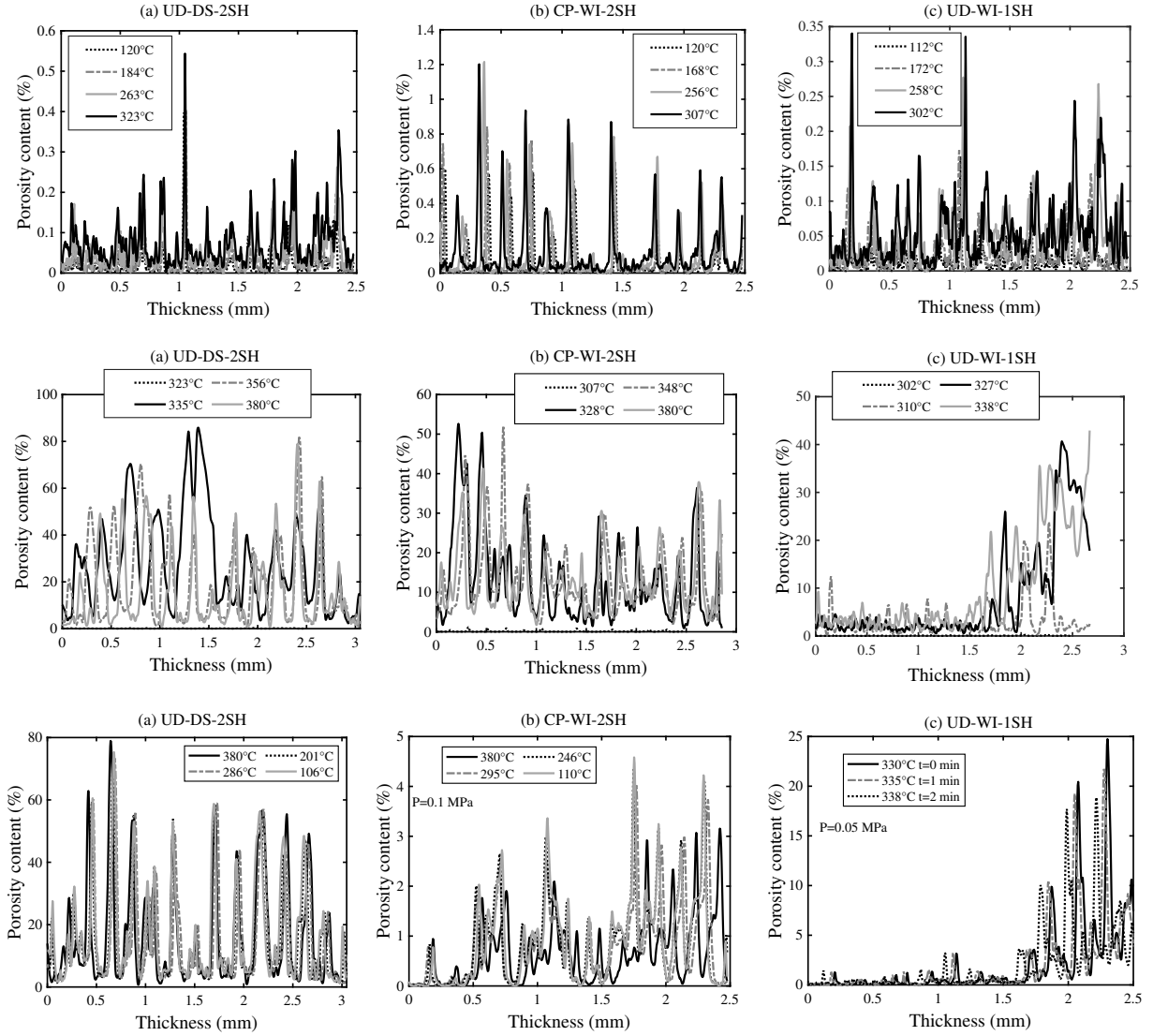
Figure 11: Evolution of the spatial distribution through the sample thickness porosity \phi_z during stage 1 (a-c), stage 2 (d-f) and stage 3 (g-i) of the deconsolidation experiments UD-DS-2SH (a,d,g), CP-WI-2SH (b,e,h) and UD-WI-1SH (c,f,i).
