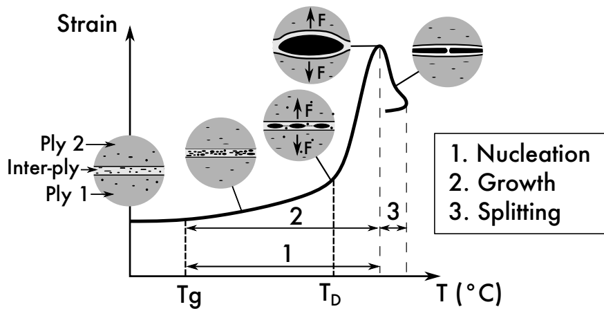
Figure 16: Schematic representation of deconsolidation process in unidirectional prepreg-based TPC laminates.
