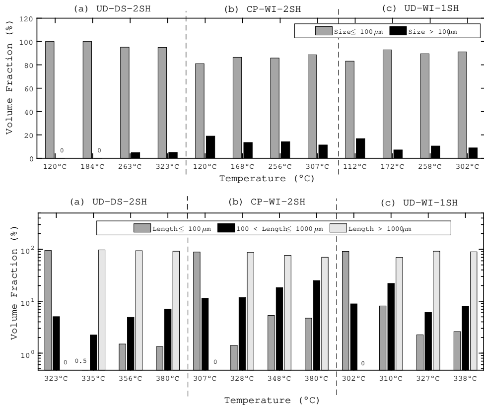
Figure 14: Volume fraction of small, medium and large-sized pores during stage 1 (a-c) and stage 2 (d-f): UD-DS-2SH (a,d), CP-WI-2SH (b,e) and UD-WI-1SH (c,f) samples.
