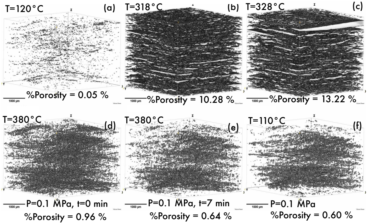
Figure 8: Time evolution of the porosity in a ROI of 3.81 \text{ mm} \times 3.81 \text{ mm} \times Z pixels during deconsolidation of an [0/90]_{4S} cross-ply laminate sample initially stored in distilled water. The black spots represent the pores.
