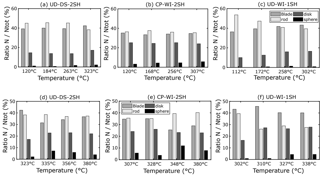
Figure 15: Distribution of pore shape during stage 1 (a-c) and stage 2 (d-f): UD-DS-2SH (a,d), CP-WI-2SH (b,e) and UD-WI-1SH (c,f) samples.
