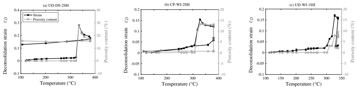
Figure 9: Deconsolidation strain \varepsilon_D and the porosity \phi of the samples vs. sample temperature estimated with the thermal model during the deconsolidation tests: test 2 on UD-DS-2SH (a), test 3 on CP-WI-2SH (b) and test 4 on UD-WI-1SH (c). The dashed circles indicate characteristic temperatures used later for microstructural analysis during deconsolidation.
