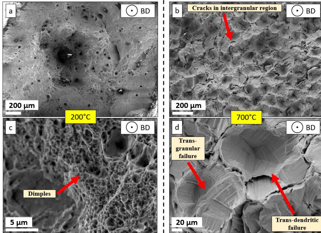
Figure 5: Fractography of LPBF Ni20Cr samples tested (a)-(b) 200°C, and (c)-(d) 700°C.
