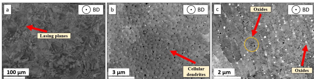
Figure 1: (a) General initial grain structure in XY plane, (b) Cellular dendritic structures and (c) Initial dislocation structures in cells of LPBFed Ni20Cr alloy using SEM (ECCI).
