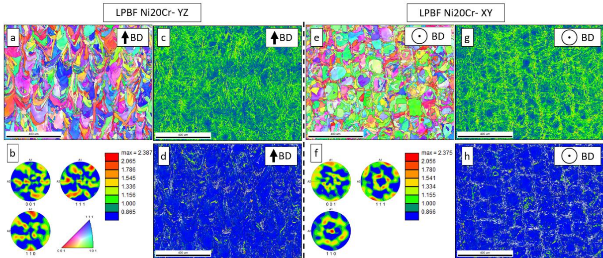
Figure 2: EBSD Inverse pole figure maps (a-e), PF maps with maximum texture intensities (b-f) with KAM (c-g) and GND maps (d-h) of the LPBF Ni20Cr in YZ and XY planes.
