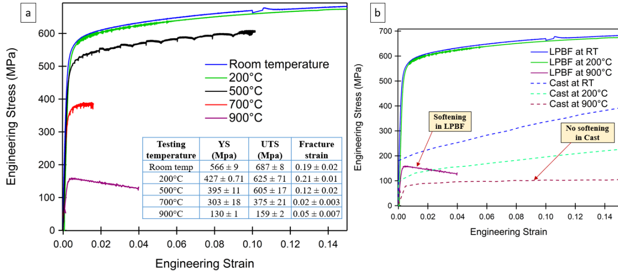
Figure 3: (a) Stress-Strain curves of LPBF Ni20Cr at room temperature, 200°C, 500°C, 700°C and 900°C with YS, UTS and fracture strain values; (b) Comparison of tensile curves of LPBF and Cast (from literature [4]) Ni20Cr at room temperature, 200°C and 900°C.
