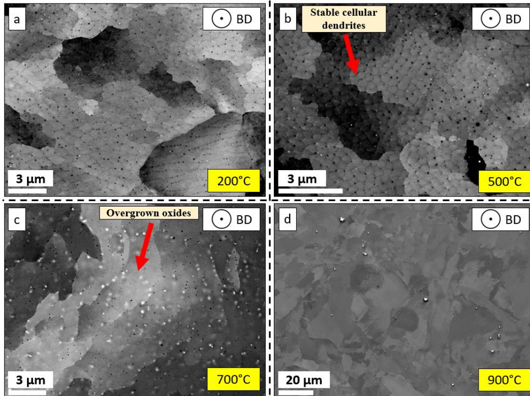
Figure 4: Microstructure of LPBF Ni20Cr alloy at pre-testing state after heat treatment for 30 minutes at (a) 200°C, (b) 500°C, (c) 700°C and (d) 900°C respectively using SEM (ECCI).
