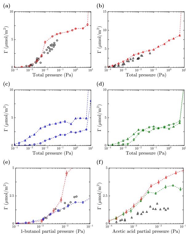
Figure 1: Average number of 1-butanol (circles) and acetic acid (triangles) molecules adsorbed on ice as a function of the pressure (note that the errors bars are smaller than the symbols), as calculated from the present GCMC simulations at 233 K, for various proportions of these two species in the gas phase. Top row: Red curves represent the results obtained for the neat (non mixed) systems. Middle row: Results obtained for the gas phase 1-butanol:acetic acid molar ratios of 25:75 (blue curves) and of 62:38 (green curves). Bottom row : Comparison between results obtained for the non-mixed and the mixed systems, for 1-butanol (left) and acetic acid (right) molecules. Lines connecting the points are only guides to the eye. Comparisons with the experimental data 8 are shown as grey symbols. Note that for the mixtures, these experimental data are available for only one species in each case, i.e., 1-butanol for the gas phase 1-butanol:acetic acid molar ratios of 25:75, and acetic acid for the gas phase 1-butanol:acetic acid molar ratios of 62:38.
