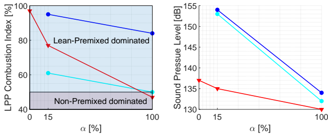
FIGURE 8: EVOLUTION IN FUNCTION OF STAGING FACTOR ( \alpha ) OF: LPP COMBUSTION INDEX (LEFT) AND SPL RIGHT) FOR V (RED), TULIP (CYAN) AND M (BLUE) FLAMES. THE SYMBOLS REPRESENT DATA POINTS OF THE SIMULATIONS.
