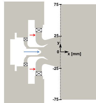
Fig. 1: 2D view of the injector at the entrance of the combustion chamber. The central blue arrow indicates the pilot injector, while the two external red arrows, the radial position of multi-point injection holes. Flow from left to right.
