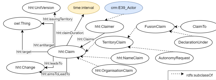
Figure 5. Scheme of the ontological module HHT-Claim
