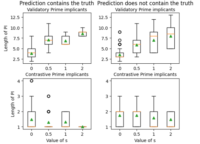
Figure 1: Explanation length according to prediction truth. Green triangles are mean values.
